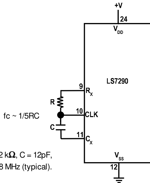
FIGURE 3. RC OSCILLATOR FOR CLOCK GENERATOR
