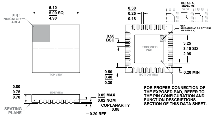
Figure 76. 32-Lead Lead Frame Chip Scale Package [LFCSFP] 5 mm x 5 mm Body and 0.75 mm Package Height (CP-32-7)
