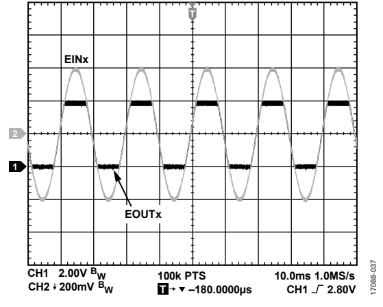
Figure 38. PGA No Phase Reversal, V_{VCOM} = V_{AVDD} = 4V , A_V = -10
