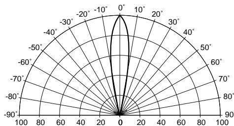
Fig. 5 Radiation Diagram
