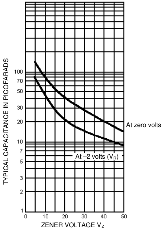
FIGURE 3 CAPACITANCE vs. V_Z CURVE
