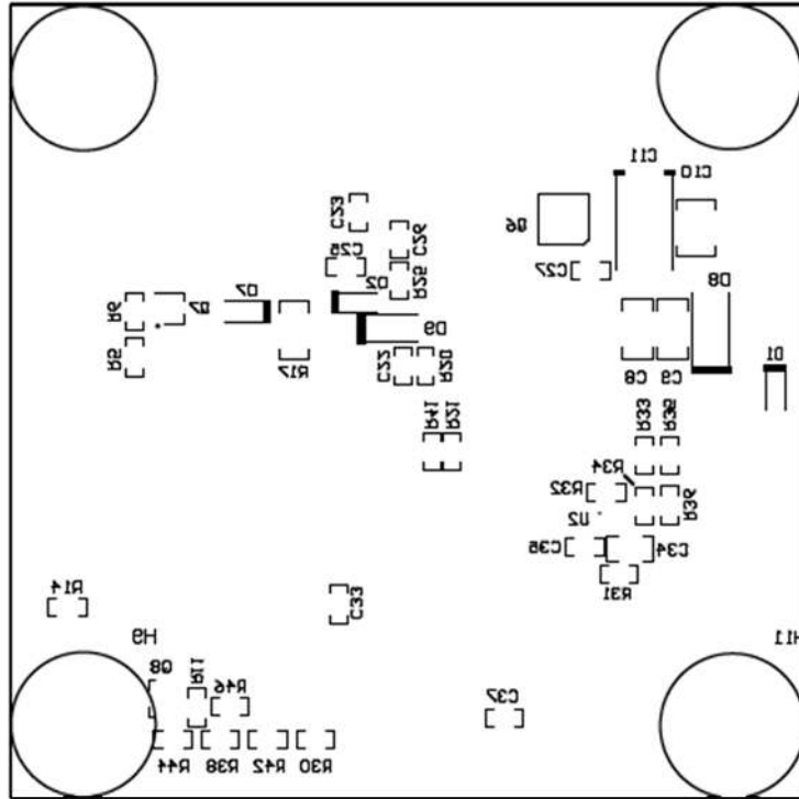
Figure 10. Bottom Assembly
