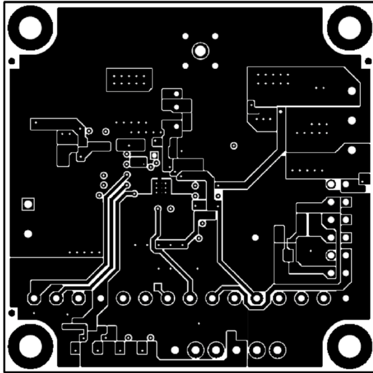
Figure 9. Bottom Layer
