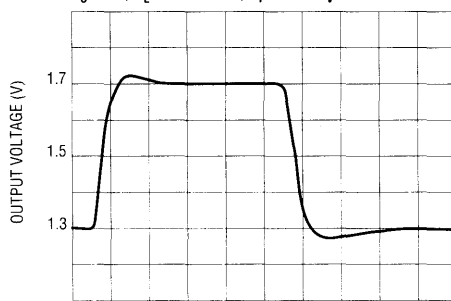
TIME (20ns/DIV)
