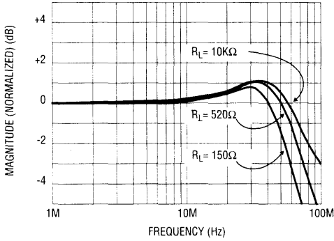
Frequency Response for Various R_L V_{CM} = 1.5V, R_F = 0\Omega, A_V = +1
