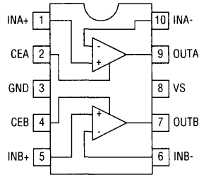
EL5246C (10-Pin MSOP)
