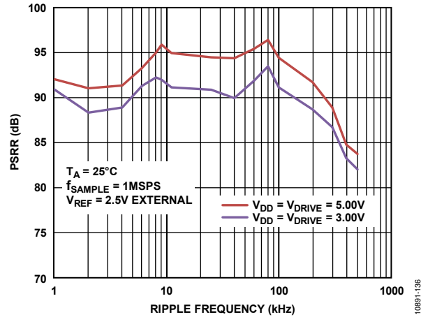
Figure 32. PSRR vs. Ripple Frequency
