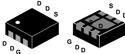
DFN2x2-6L 2EP
