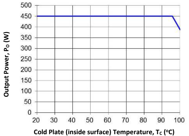
Figure 20. Derating Output Power in conduction cooling (cold plate) applications, V_{in}=48V .
