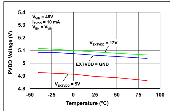
FIGURE 2-6: PVDD Voltage vs. Temperature.
