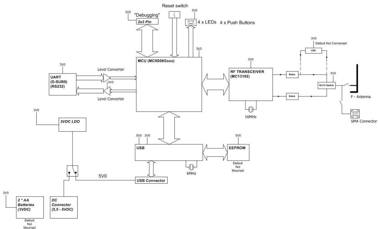
Figure 1 13192-EVB Block Diagram
