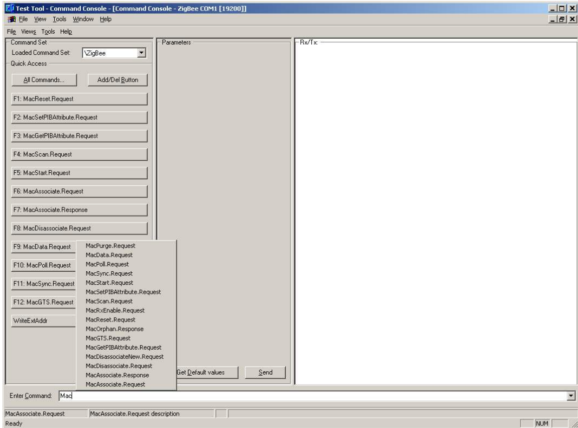
Figure 18 Command Console (MAC Command Entries)
