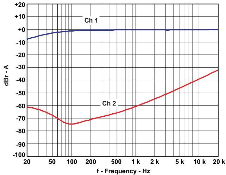
Figure 16. Channel Separation (1-2)
