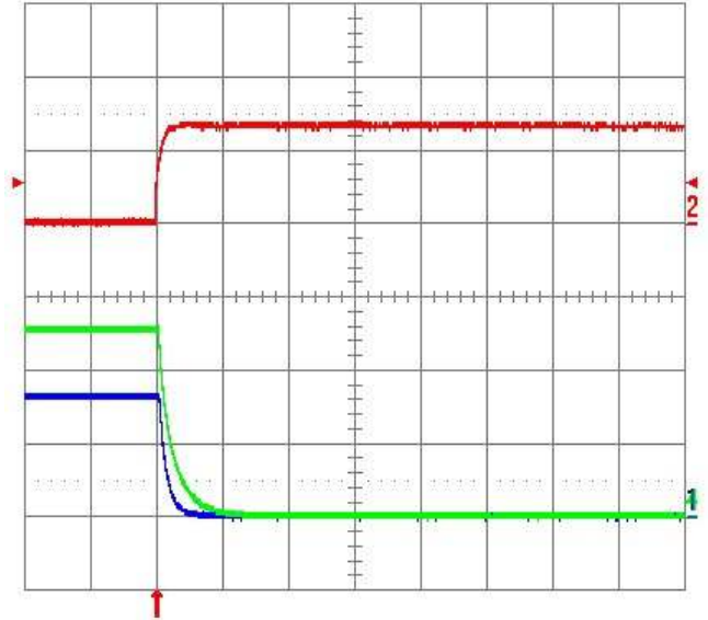
Fig. 14: Turn-off transient for V_{out} = 3.3\text{ V} and 5.0\text{ V} with the removal of SEQ/ENA signal at full rated load current (resistive) and 1\ \mu\text{F} external capacitance at V_{in} = 12\text{ V} . SEQ/ENA pins are tied together. Top Trace: SEQ/ENA Signal (5 V/div.); Middle Trace: Output Voltage of 5V POL (2V/div.); Bottom Trace: Output Voltage of 3.3V POL (2 V/div.); Time Scale: 2 ms/div.
