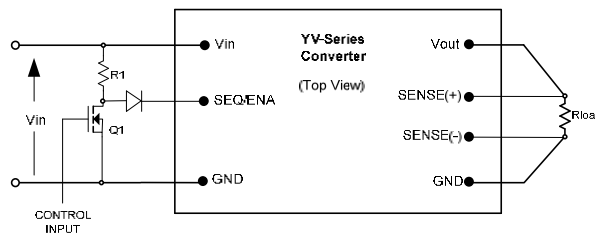
Fig. A: Circuit configuration for ON/OFF function.
