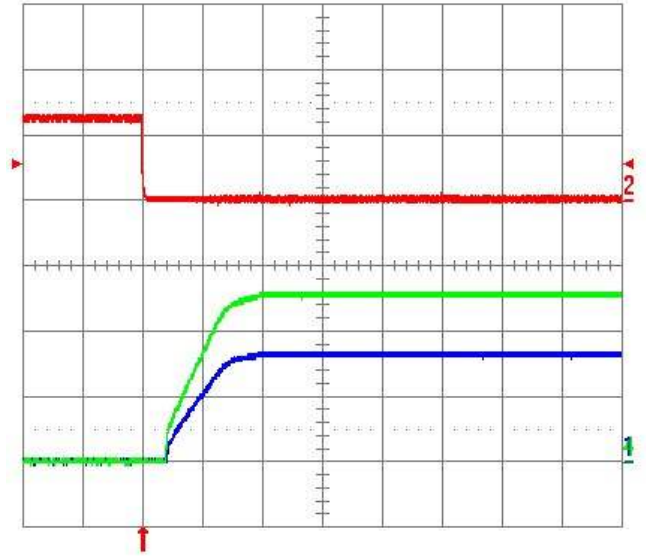
Fig. 12: Turn-on transient for V_{out} = 3.3\text{ V} and 5.0\text{ V} with the application of SEQ/ENA signal at full rated load current (resistive) and 1\ \mu\text{F} external capacitance at V_{in} = 12\text{ V} . SEQ/ENA pins are tied together. Top Trace: SEQ/ENA Signal (5 V/div.); Middle Trace: Output Voltage of 5V POL (2V/div.); Bottom Trace: Output Voltage of 3.3V POL (2 V/div.); Time Scale: 2 ms/div.
