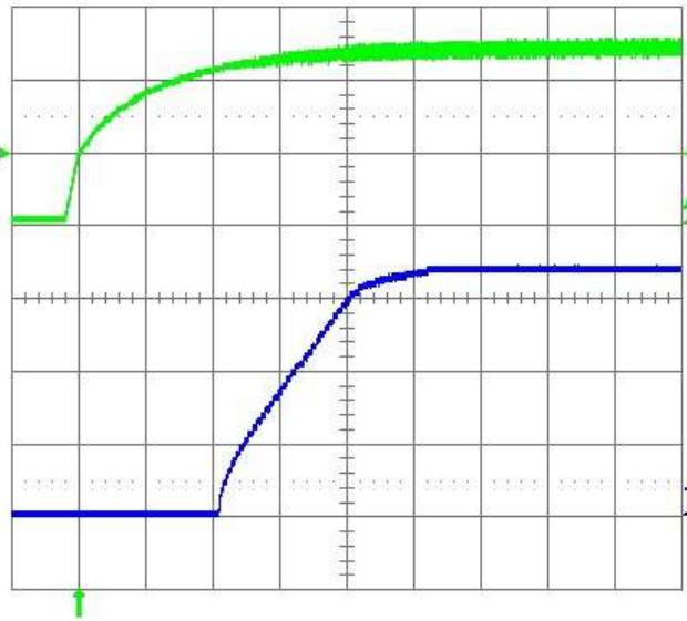
Fig. 13: Turn-on transient for V_{out} = 3.3\text{ V} with the application of the input voltage at full rated load current (resistive) and 1\ \mu\text{F} external capacitance at V_{in} = 12\text{ V} . Top Trace: Input Voltage Signal (5 V/div.); Bottom Trace: Output Voltage (1 V/div.); Time Scale: 1 ms/div.
