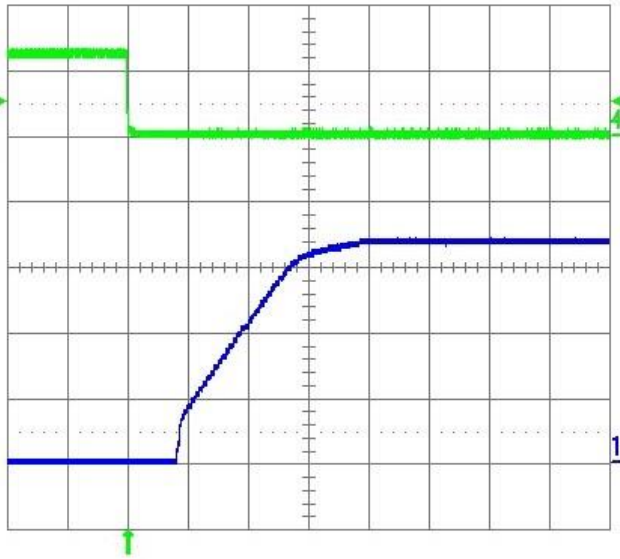
Fig. 11: Turn-on transient for V_{out} = 3.3\text{ V} with the application of SEQ/ENA signal at full rated load current (resistive) and 1\ \mu\text{F} external capacitance at V_{in} = 12\text{ V} . Top Trace: SEQ/ENA Signal (5 V/div.); Bottom Trace: Output Voltage (1 V/div.); Time Scale: 1 ms/div.
