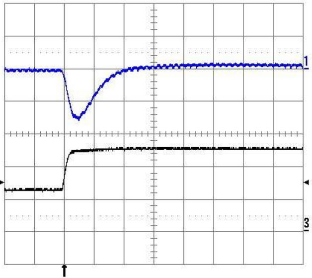
Fig. 17: Output voltage response for V_{out} = 3.3 V to positive load current step change from 12.5 A to 25 A with slew rate of 5 A/ \mu s at V_{in} = 12 V. Top Trace: Output Voltage (100 mV/div.); Bottom Trace: Load Current (10 A/div.) C_o = 1 \mu F ceramic. Time Scale: 10 \mu s/div.
