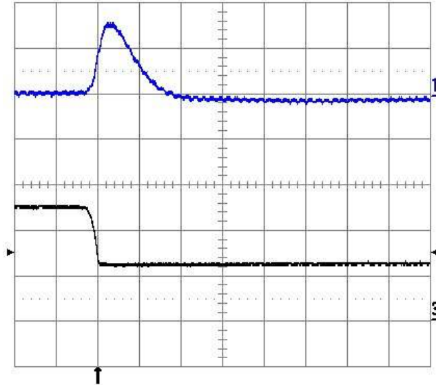
Fig. 18: Output voltage response for V_{out} = 3.3 V to negative load current step change from 25 A to 12.5 A with slew rate of -5 A/ \mu s at V_{in} = 12 V. Top Trace: Output Voltage (100 mV/div.); Bottom Trace: Load Current (10 A/div.) C_o = 1 \mu F ceramic. Time Scale: 10 \mu s/div.
