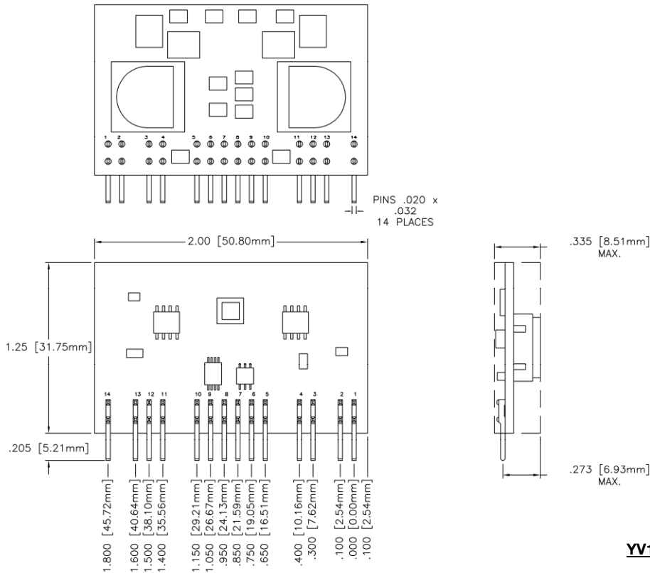
Through-hole – SIP
