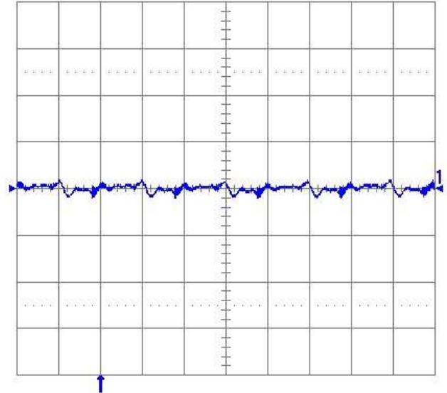
Fig. 16: Output voltage ripple (20 mV/div.) at full rated load current into a resistive load with external capacitance 1 \mu F ceramic and V_{in} = 12 V for V_{out} = 1.2 V. Time Scale: 1 \mu s/div.
