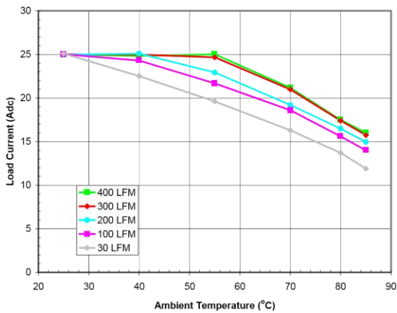
Fig. 9: Available load current vs. ambient temperature and airflow rates for V_{out} = 1.8\text{ V} with V_{in} = 12\text{ V} , and maximum MOSFET temperature \leq 110\text{ }^{\circ}\text{C} . Horizontal Orientation (Airflow from Vin pin to GND pin.)
