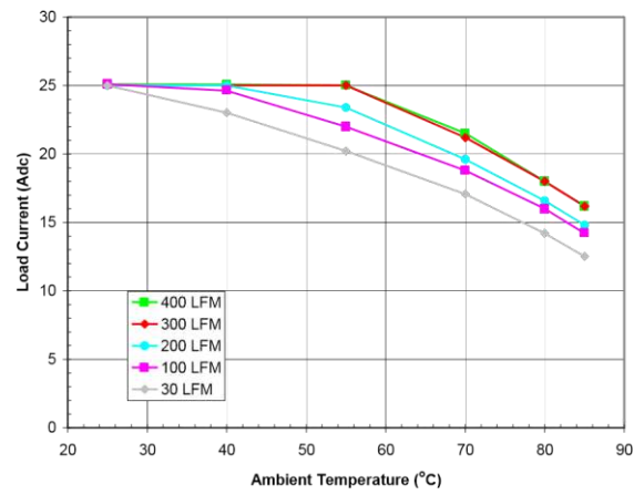
Fig. 10: Available load current vs. ambient temperature and airflow rates for V_{out} = 1.2\text{ V} with V_{in} = 12\text{ V} , and maximum MOSFET temperature \leq 110\text{ }^{\circ}\text{C} . Horizontal Orientation (Airflow from Vin pin to GND pin.)
