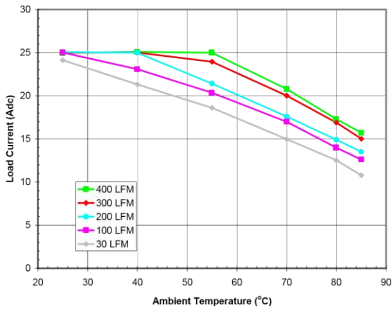
Fig. 7: Available load current vs. ambient temperature and airflow rates for V_{out} = 5.0\text{ V} with V_{in} = 12\text{ V} , and maximum MOSFET temperature \leq 110\text{ }^{\circ}\text{C} . Horizontal Orientation (Airflow from Vin pin to GND pin.)
