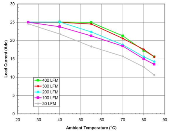
Fig. 8: Available load current vs. ambient temperature and airflow rates for V_{out} = 3.3\text{ V} with V_{in} = 12\text{ V} , and maximum MOSFET temperature \leq 110\text{ }^{\circ}\text{C} . Horizontal Orientation (Airflow from Vin pin to GND pin.)
