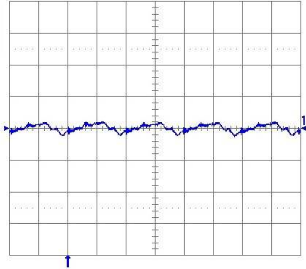
Fig. 15: Output voltage ripple (20 mV/div.) at full rated load current into a resistive load with external capacitance 1 \mu F ceramic and V_{in} = 12 V for V_{out} = 3.3 V. Time Scale: 1 \mu s/div.
