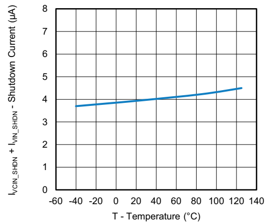
Fig. 44 - Shutdown Current vs. Junction Temperature
