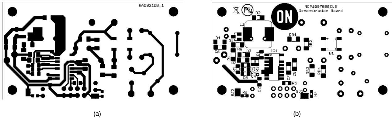
Figure 3. NCP10970BGEVB – Bottom Side – (a) Layer, (b) Components
