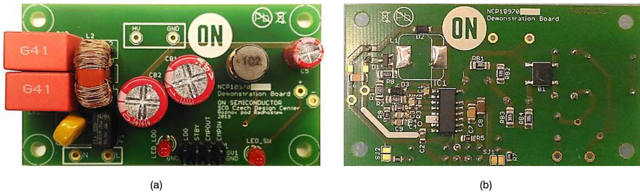
Figure 4. NCP10970BGEVB Board Photo – (a) Top Side, (b) Bottom Side
