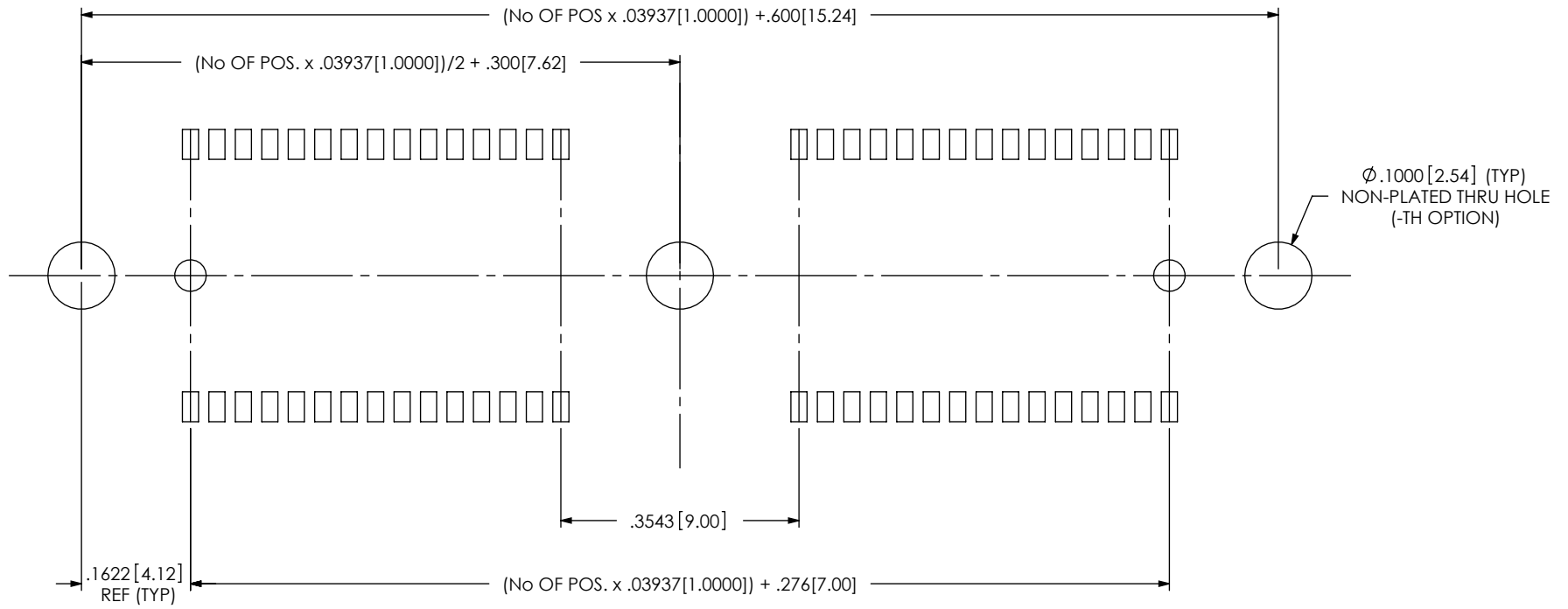
FIG 2 FOR -40 AND -50 POS (THREADED)
