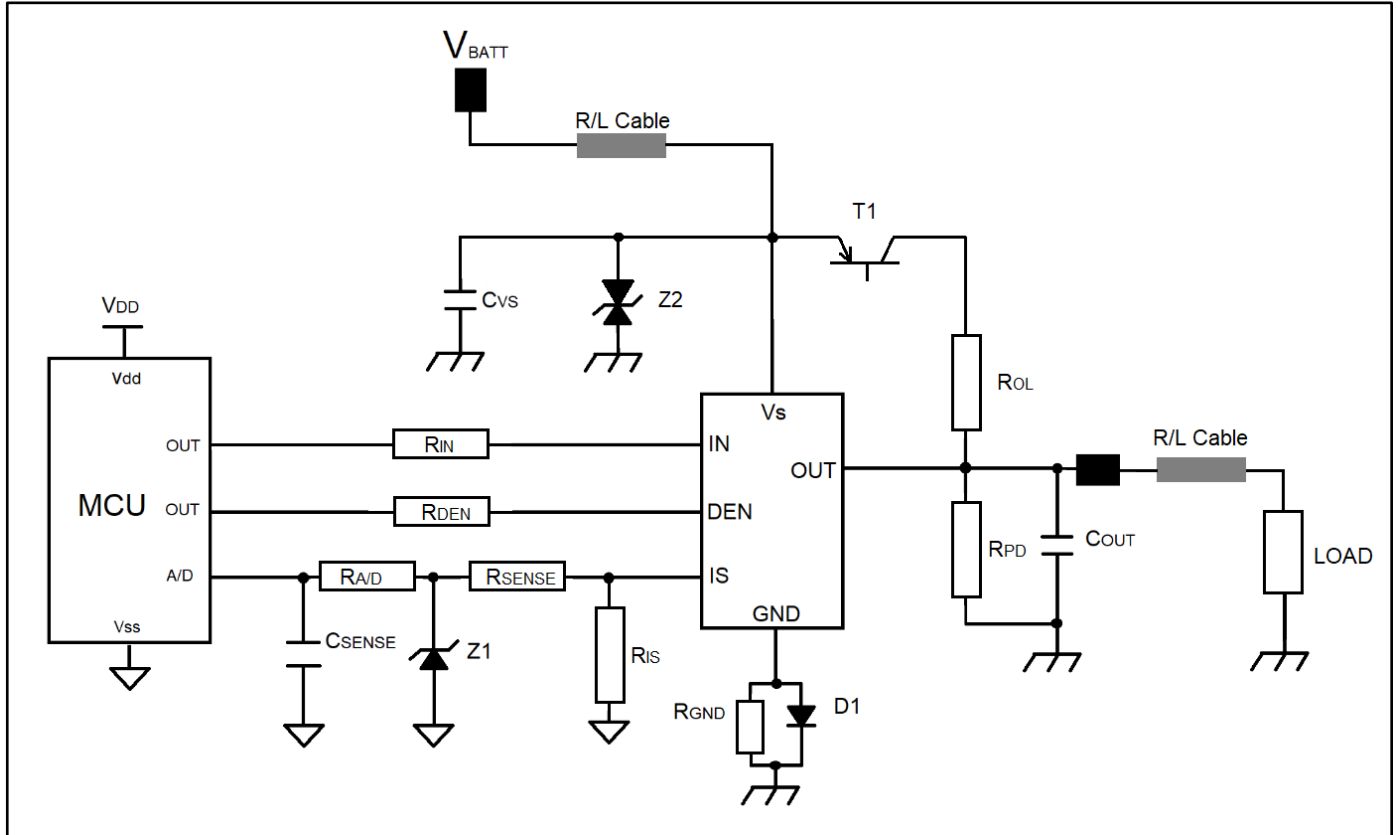
Figure 38. Application Diagram
