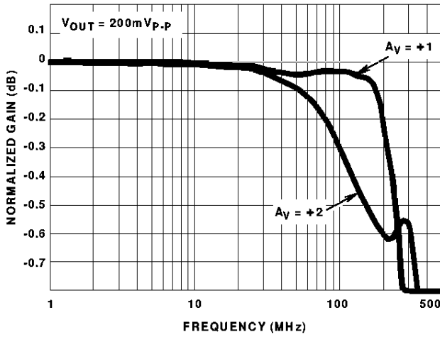
FIGURE 15. GAIN FLATNESS
