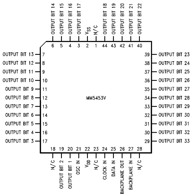
Figure 5. Top View See Package Number FN0044A
