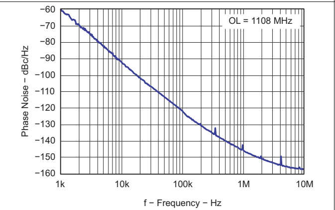
Figure 77. Open Loop VCO Phase Noise
