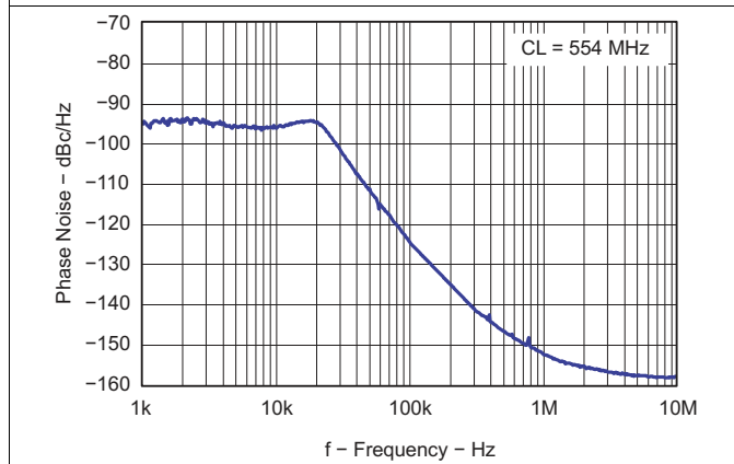
Figure 78. Closed Loop VCO Phase Noise
