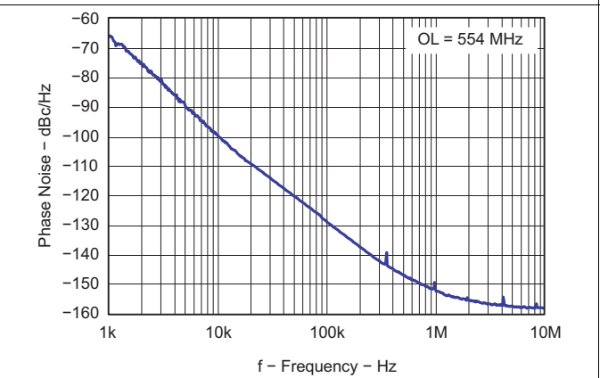
Figure 79. Open Loop VCO Phase Noise
