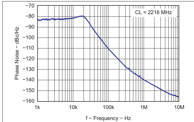
Figure 74. Closed Loop VCO Phase Noise
