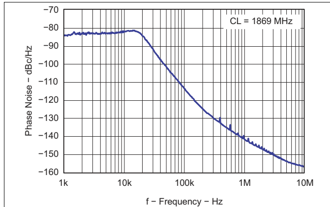
Figure 38. Closed Loop VCO Phase Noise
