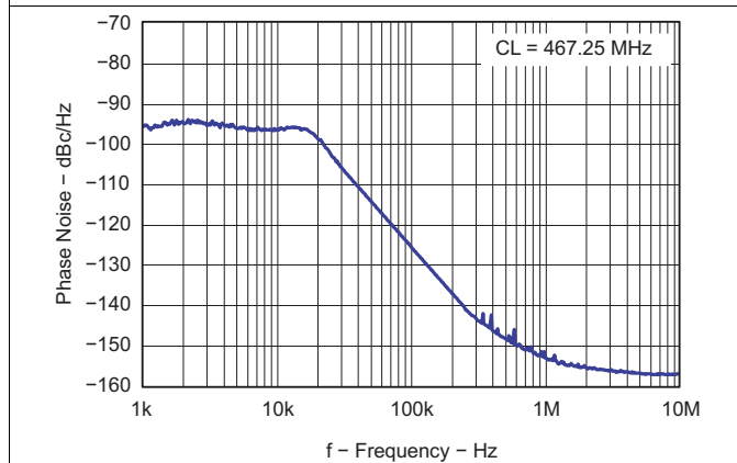
Figure 42. Closed Loop VCO Phase Noise
