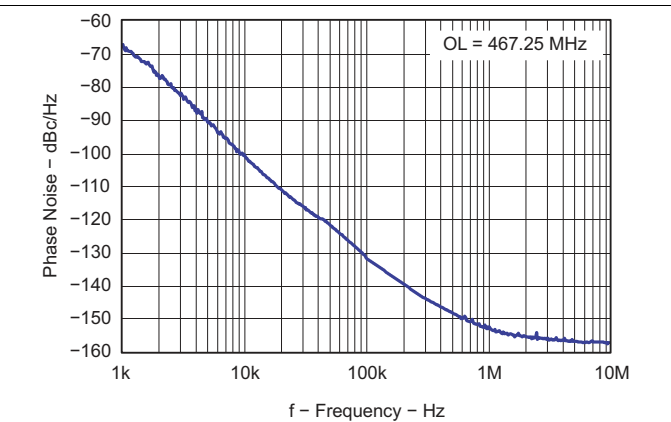
Figure 43. Open Loop VCO Phase Noise
