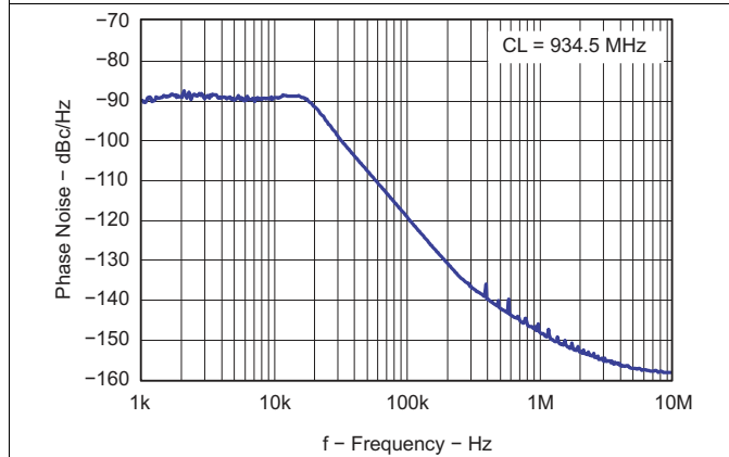
Figure 40. Closed Loop VCO Phase Noise
