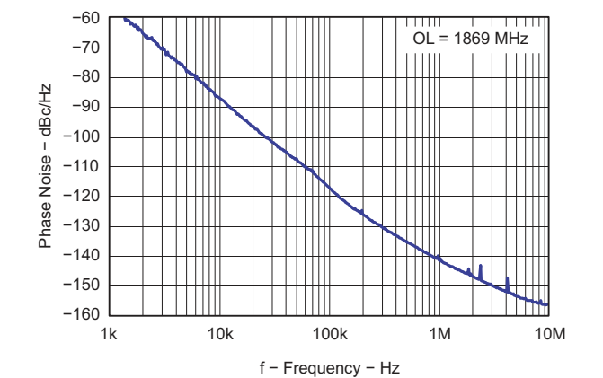
Figure 39. Open Loop VCO Phase Noise
