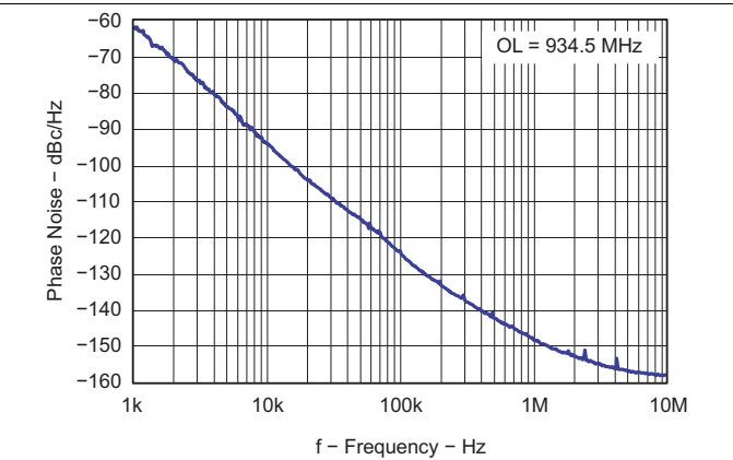
Figure 41. Open Loop VCO Phase Noise
