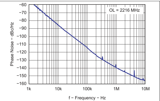
Figure 75. Open Loop VCO Phase Noise
