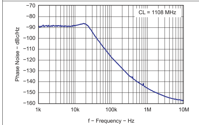
Figure 76. Closed Loop VCO Phase Noise
