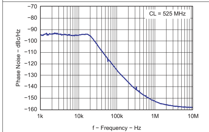
Figure 69. Closed Loop VCO Phase Noise
