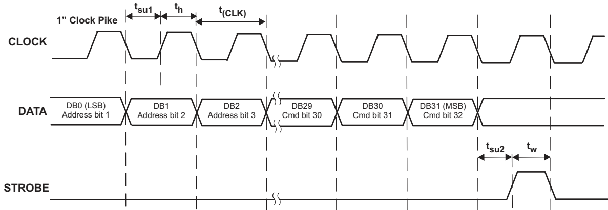
Figure 83. Serial Programming Timing Diagram
