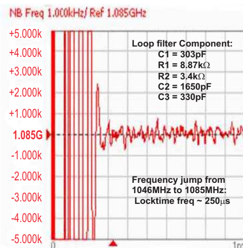
Figure 88. Frequency Locktime
