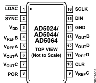
Figure 7. 16-Lead TSSOP (RU-16) Pin Configuration
