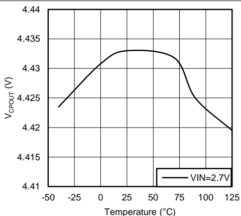
Figure 8. Charge Pump 2X Mode V_{CP\text{OUT}} vs Temperature
