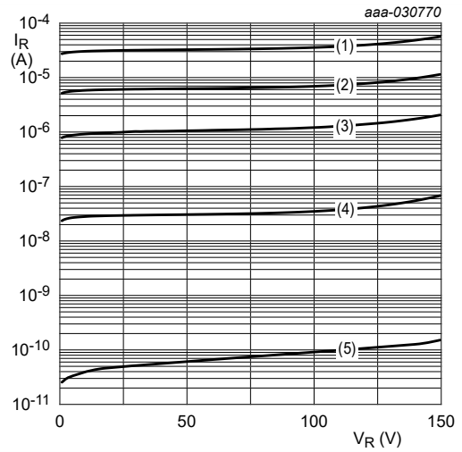
pulsed condition (1) T_j = 175\text{ °C} (2) T_j = 150\text{ °C} (3) T_j = 125\text{ °C} (4) T_j = 85\text{ °C} (5) T_j = 25\text{ °C}
