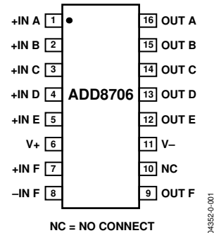
Figure 1. 16-Lead TSSOP
