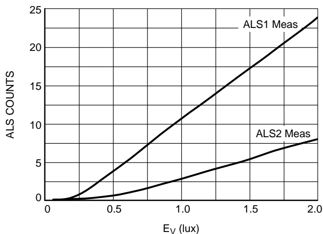
Figure 9. ALS1 Linearity 0–2 lux
