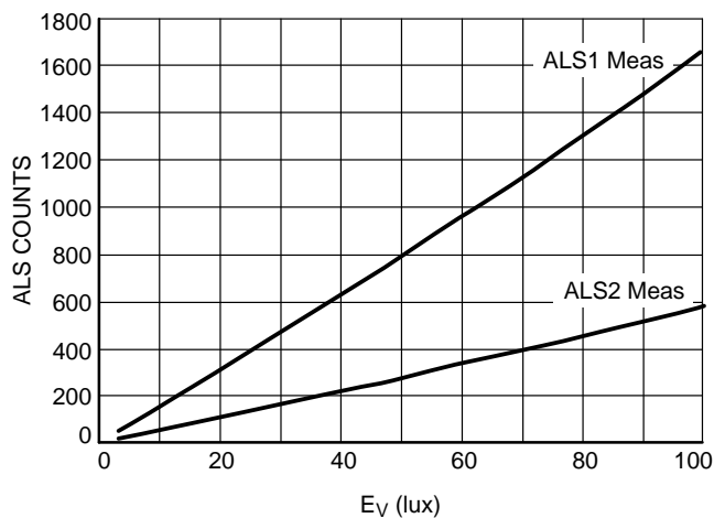
Figure 7. ALS1 Linearity 0–100 lux
