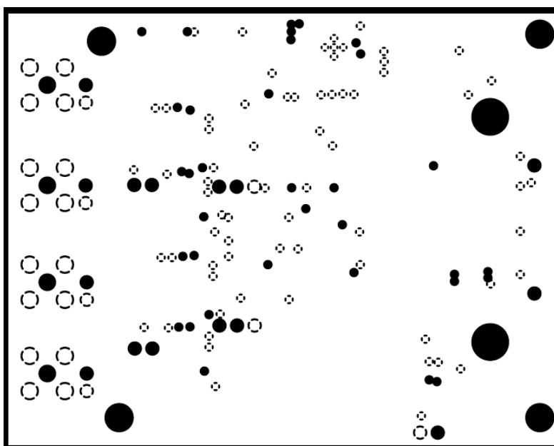
Figure 14. ADS8353-Q1EVM PCB Layer 2: GND Plane
