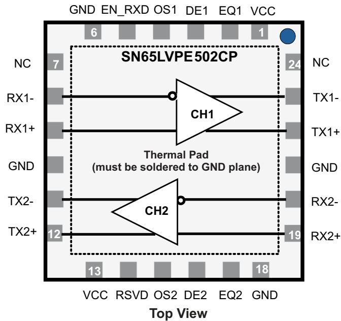
Figure 8. Flow-Through Pin-Out
