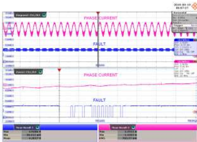
Figure 60 – System Thermal Fault, 5000 RPM, 200 W.
