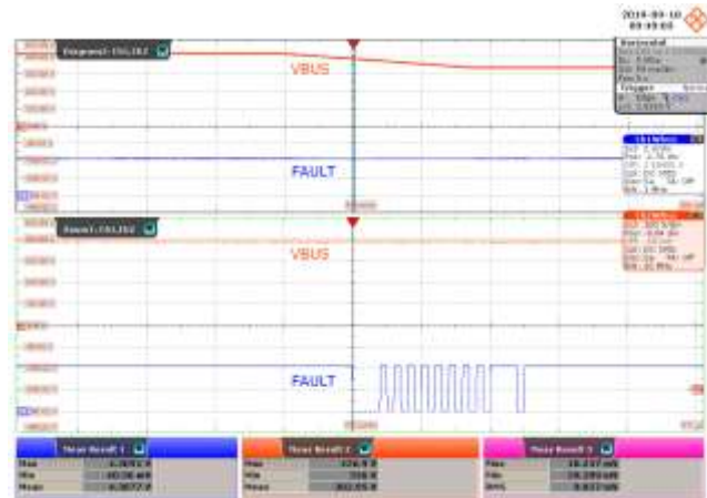
Figure 57 – OVP clear, 425 V to 340 V.
