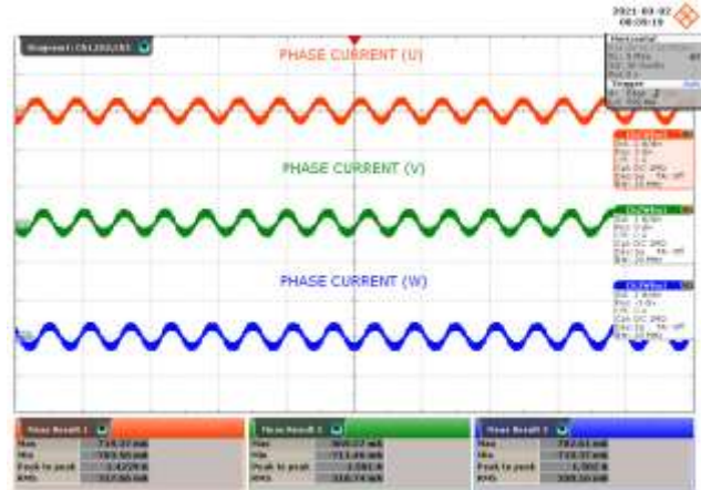
Figure 25 – Phase Current at 100 W Load.
