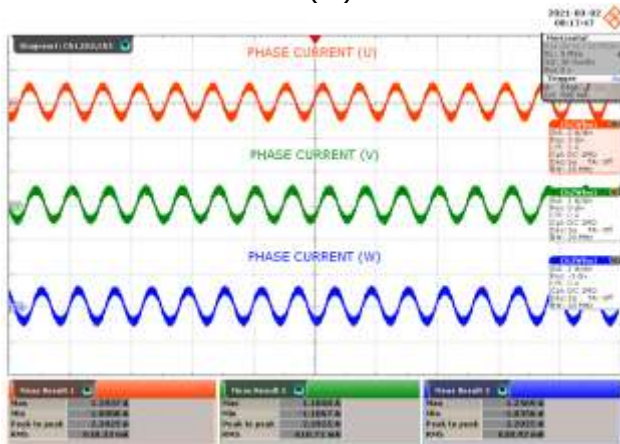
Figure 26 – Phase Current at 200 W Load.
