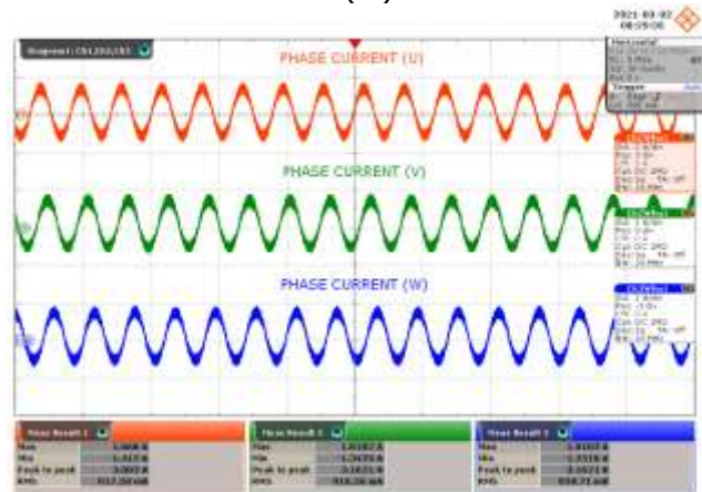
Figure 27 – Phase Current at 300 W Load.
