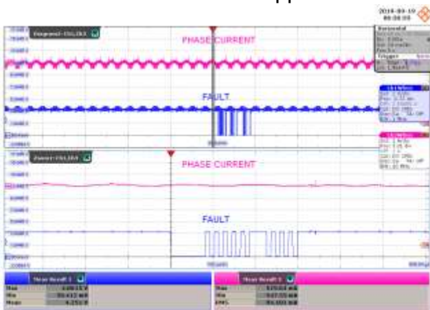
Figure 47 – Thermal Warning at Light Load. CH3: I_{PHASE} , 1 A / div. CH1: V_{FAULT} , 2 V / div. Time Scale: 20 ms / div. Time Scale (Zoomed Area): 100 \mu s / div. FAULT Flag/Reading = 0000100.
