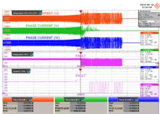
Figure 63 – At Stalled Condition, 300 W Load.
