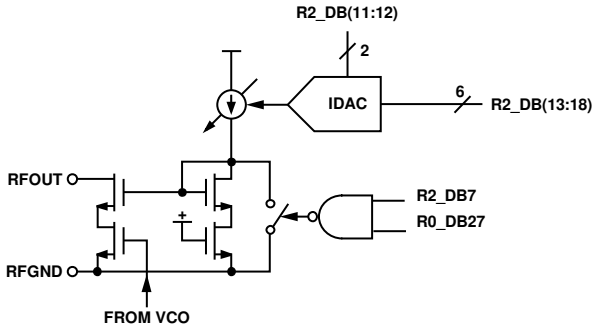
Figure 39. PA Configuration
