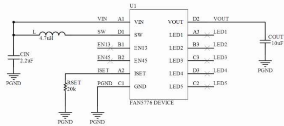
Figure 28. Schematic for Recommended Layout
