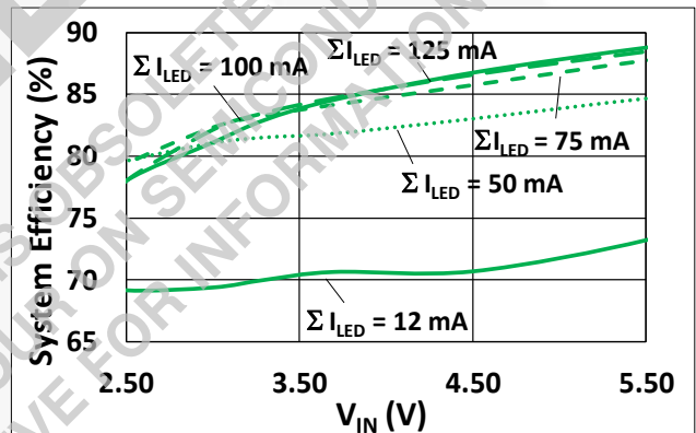
Figure 7. Total Efficiency vs. Input Voltage vs. Total LED Current
