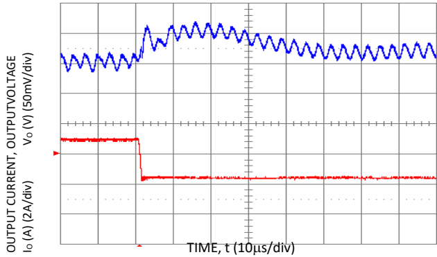
Figure 13. Transient Response to Dynamic Load Change from 100% of full load ( V_o = 3.3Vdc , C_{ext} = 2 \times 150 \mu F Polymer Capacitors).
