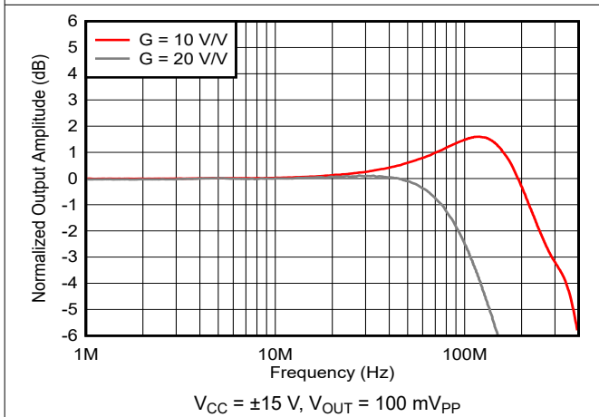
Figure 6-3. Frequency Response vs Gain
