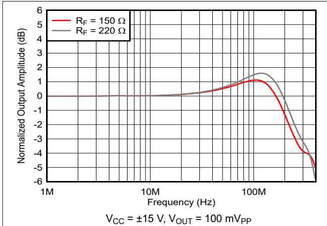
Figure 6-1. Frequency Response vs Feedback Resistance
