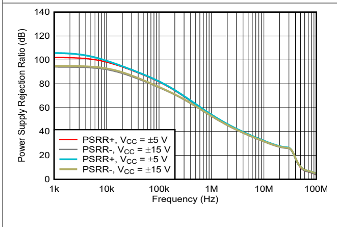
Figure 6-9. Power-Supply Rejection Ratio vs Frequency
