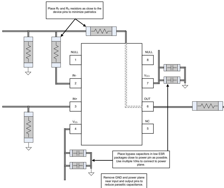
Figure 8-4. Layout Recommendations
