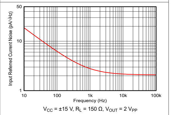
Figure 6-12. Input-Referred Current Noise vs Frequency
