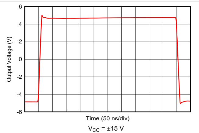
Figure 6-22. 10-V Step Response
