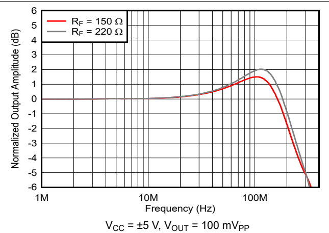
Figure 6-2. Frequency Response vs Feedback Resistance
