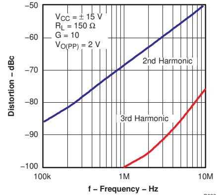
Figure 6-38. Distortion vs Frequency
