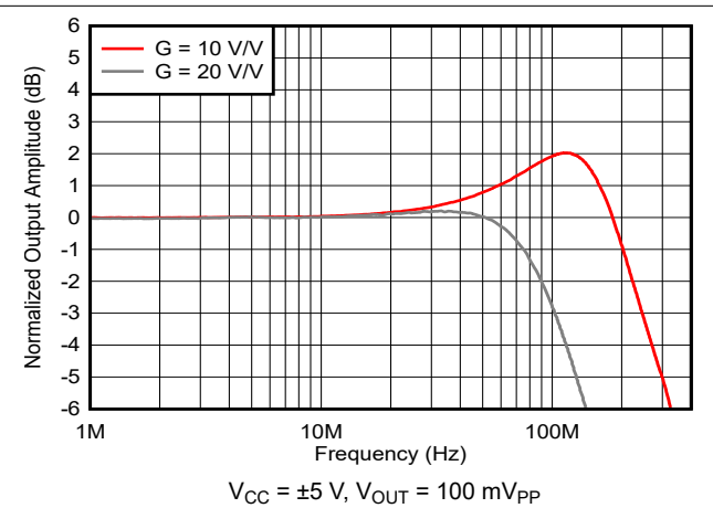
Figure 6-4. Frequency Response vs Gain
