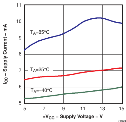
Figure 6-53. Supply Current vs Supply Voltage
