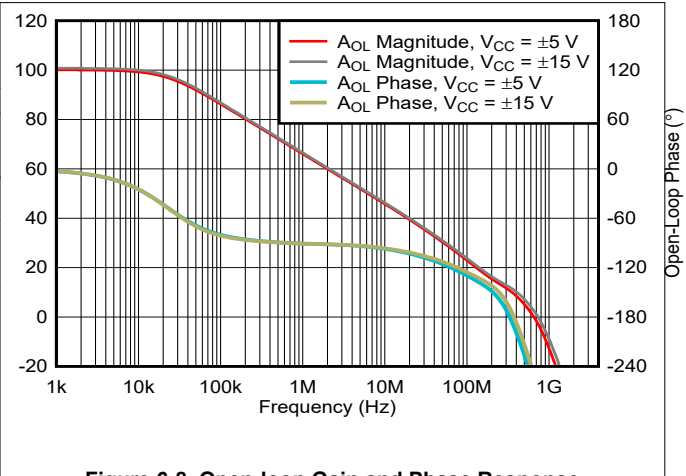
Figure 6-8. Open-loop Gain and Phase Response
