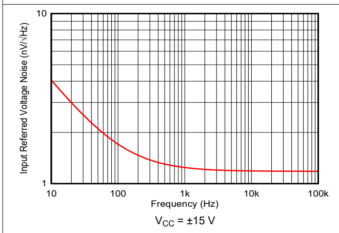
Figure 6-11. Input-Referred Voltage Noise vs Frequency
