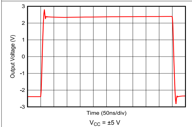
Figure 6-21. 5-V Step Response
