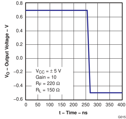
Figure 6-44. 1-V Step Response
