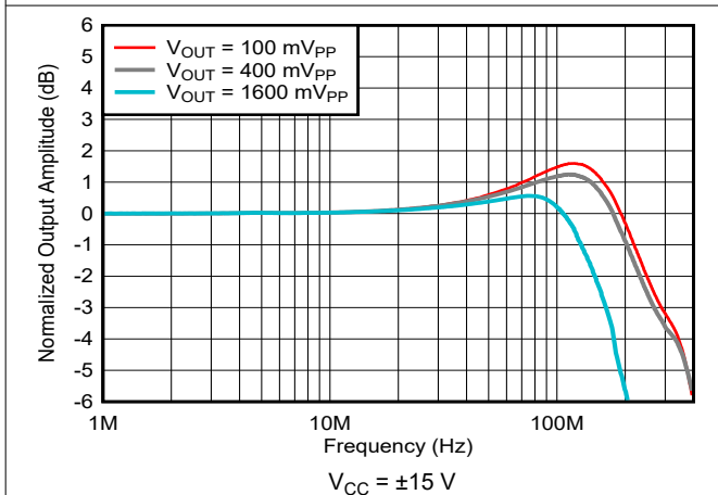
Figure 6-5. Large-Signal Frequency Response
