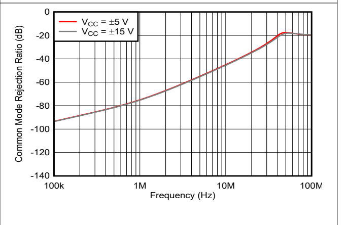
Figure 6-10. Common-Mode Rejection Ratio vs Frequency
