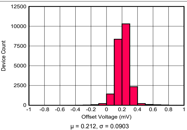
Figure 6-24. Voltage Offset Distribution
