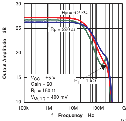
Figure 6-43. Output Amplitude vs Frequency
