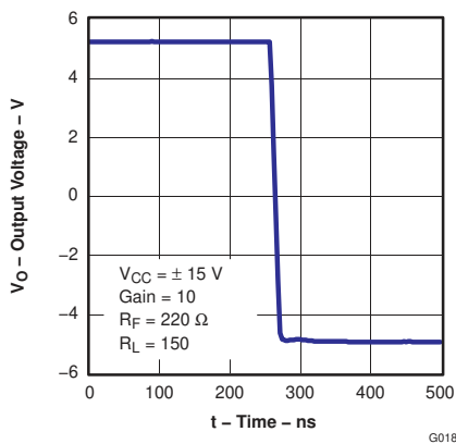
Figure 6-47. 10-V Step Response
