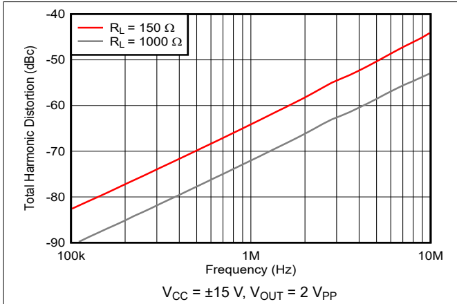
Figure 6-19. Total Harmonic Distortion vs Frequency
