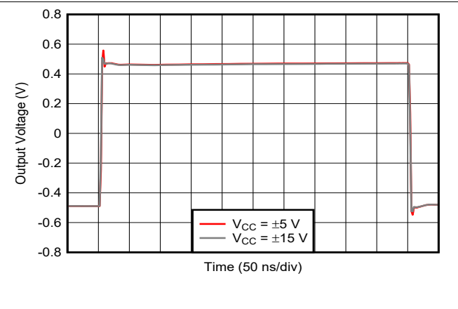
Figure 6-20. 1-V Step Response
