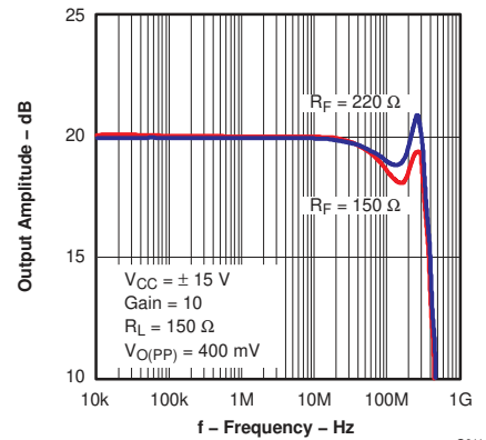
Figure 6-40. Output Amplitude vs Frequency
