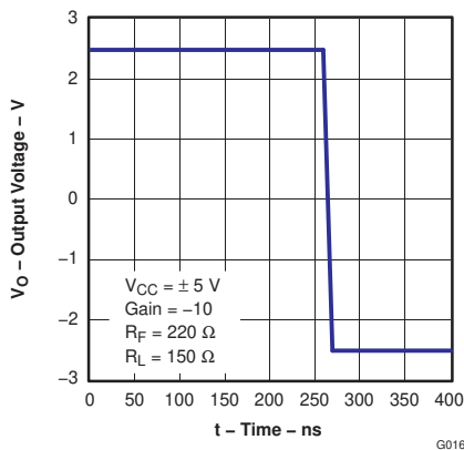
Figure 6-45. 5-V Step Response
