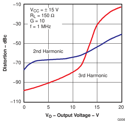
Figure 6-35. Distortion vs Output Voltage
