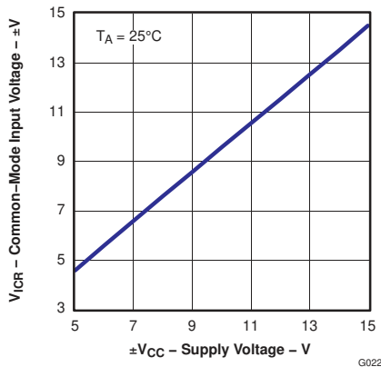
Figure 6-51. Common-mode Input Voltage vs Supply Voltage
