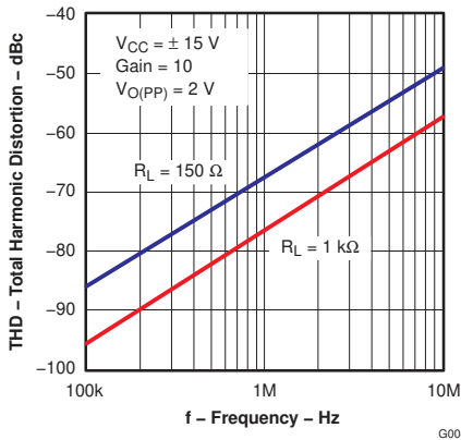
Figure 6-33. Total Harmonic Distortion vs Frequency
