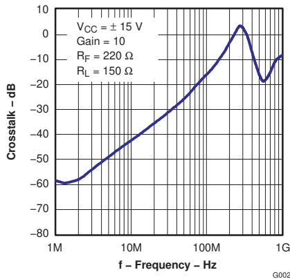
Figure 6-31. Crosstalk vs Frequency
