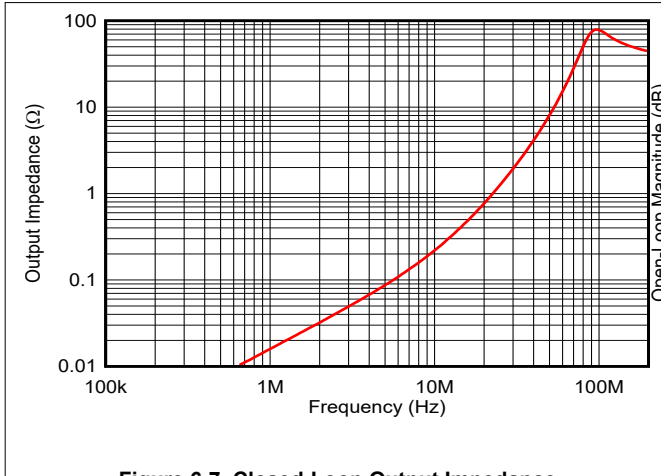
Figure 6-7. Closed-Loop Output Impedance
