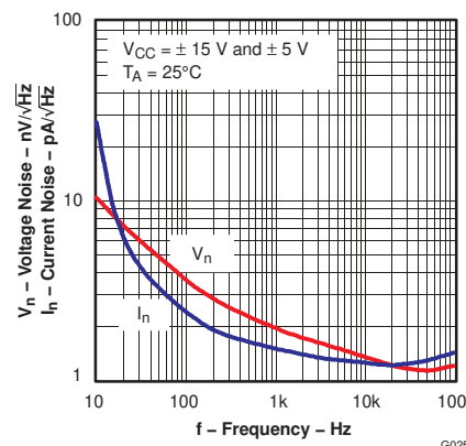
Figure 6-54. Voltage and Current Noise vs Frequency
