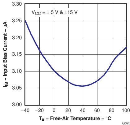
Figure 6-49. Input Bias Current vs Free-air Temperature
