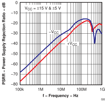
Figure 6-55. Power Supply Rejection Ratio vs Frequency
