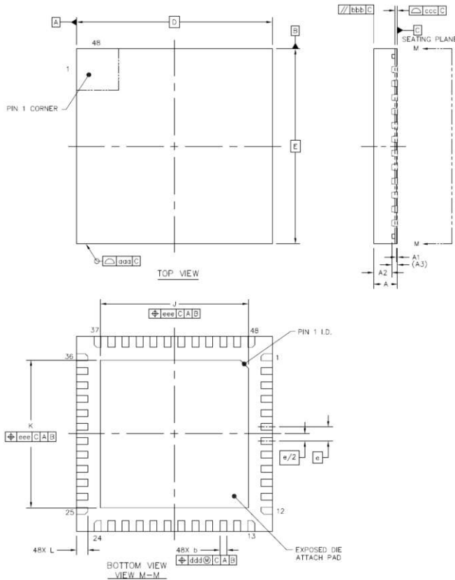
Figure 19.1 Dimensional drawings
