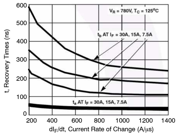
Figure 4. t_a and t_b Curves vs. di/dt
