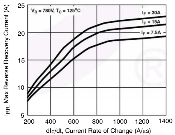
Figure 6. Maximum Reverse Recovery Current vs. di/dt
