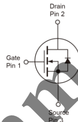
TO-251 (IPAK)
