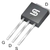
TO-251 (IPAK)
