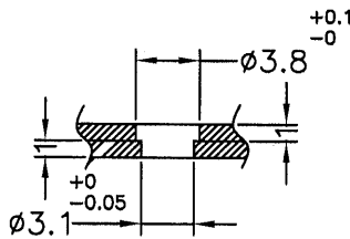
HOLE IN PANEL
