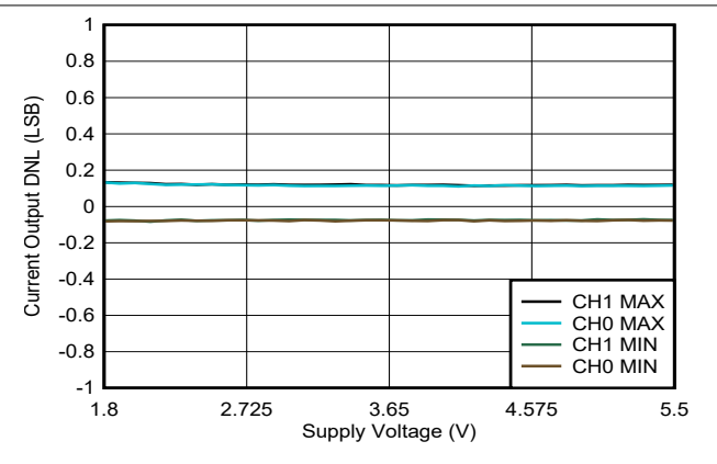
Figure 6-39. Current Output DNL vs Supply Voltage
