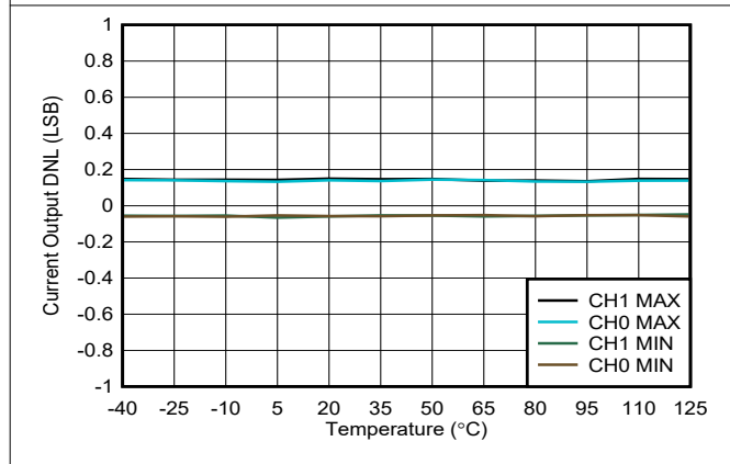
Figure 6-38. Current Output DNL vs Temperature
