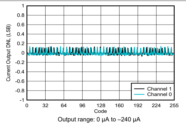
Figure 6-37. Current Output DNL vs Digital Input Code
