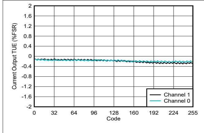
Figure 6-40. Current Output TUE vs Digital Input Code
