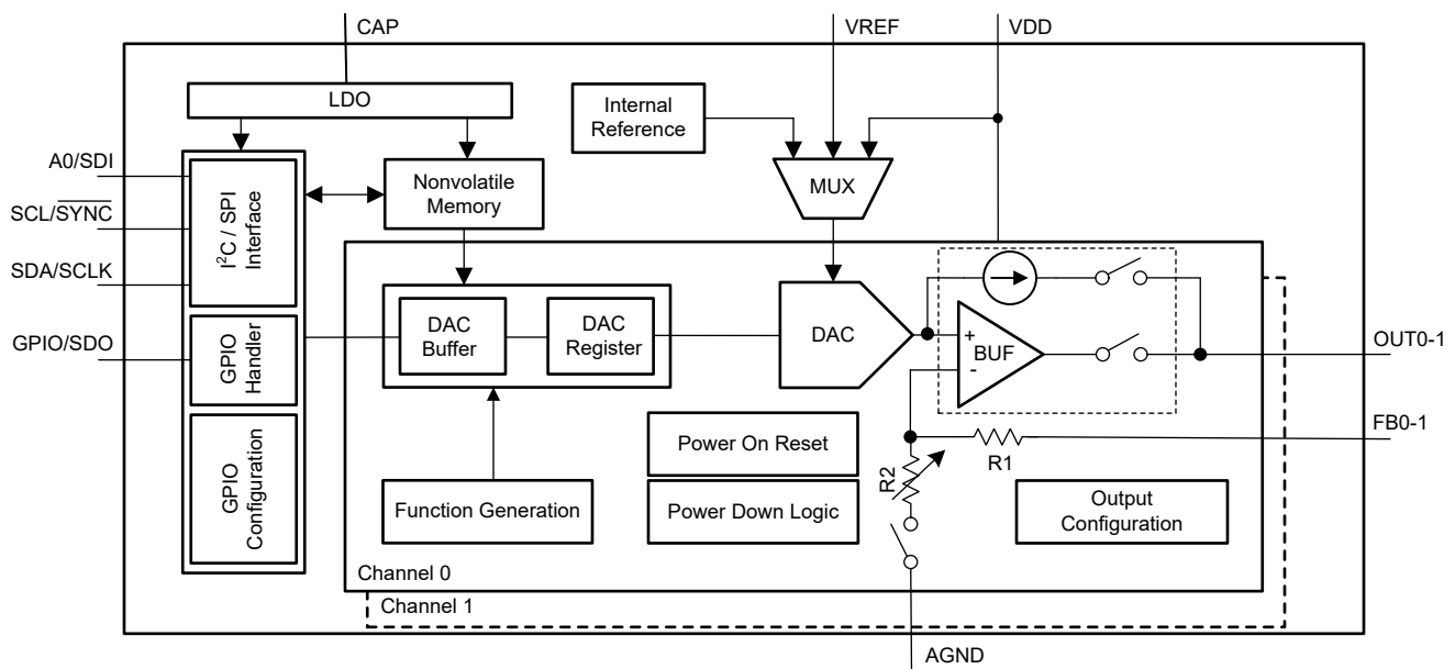
Figure 7-1. Functional Block Diagram
