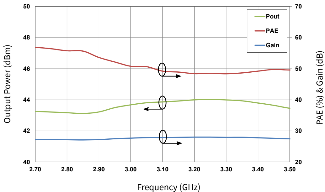
Figure 2. Output Power, Gain and PAE vs Frequency of the CMPA2735015S Measured in CMPA2735015S-AMP1 Amplifier Circuit V_{DD} = 50\text{ V}, I_{DQ} = 0.08\text{ A}, \text{Pulse Width} = 500\ \mu\text{s}, \text{Duty Cycle} = 10\%
