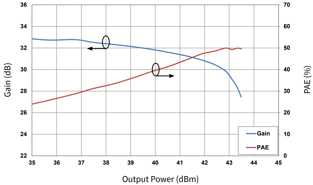
Figure 5. Gain and Power Added Efficiency vs Output Power Measured in CPA2735015S-AMP1 Amplifier Circuit V_{DD} = 50\text{ V} , I_{DQ} = 0.08\text{ A} , Frequency = 3.5 GHz
