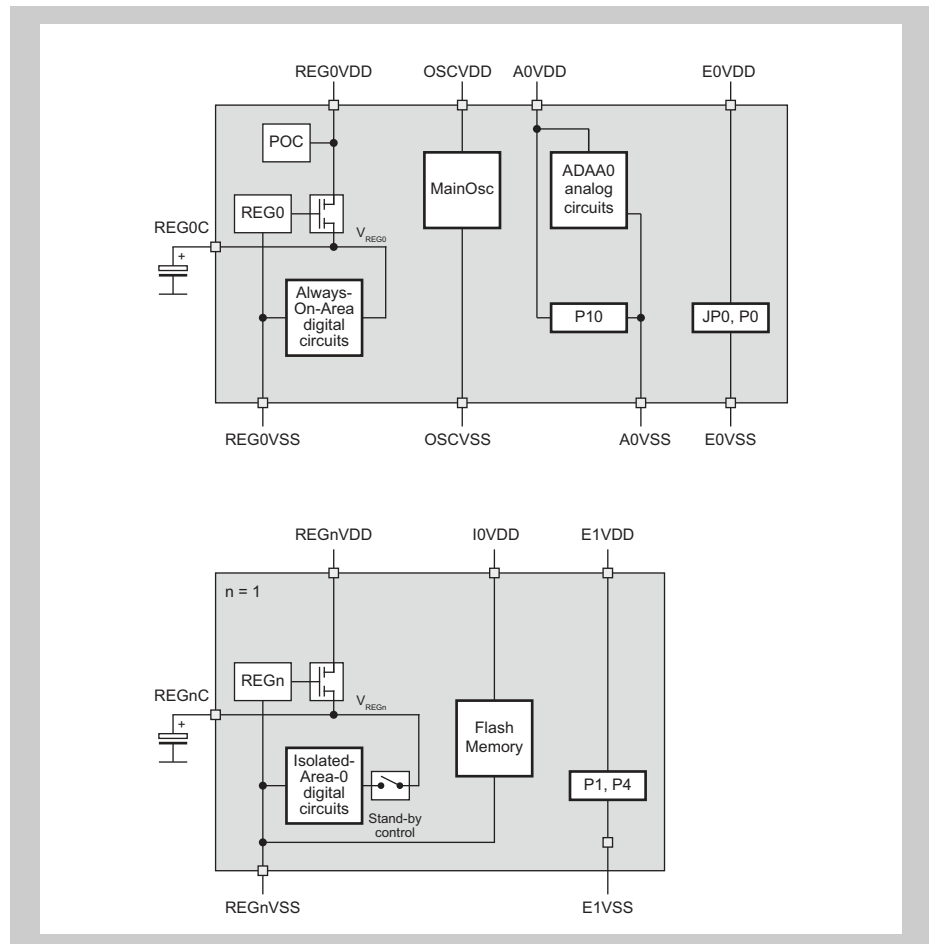
Figure 24-1 V850E2S/FE4-L power supply scheme
