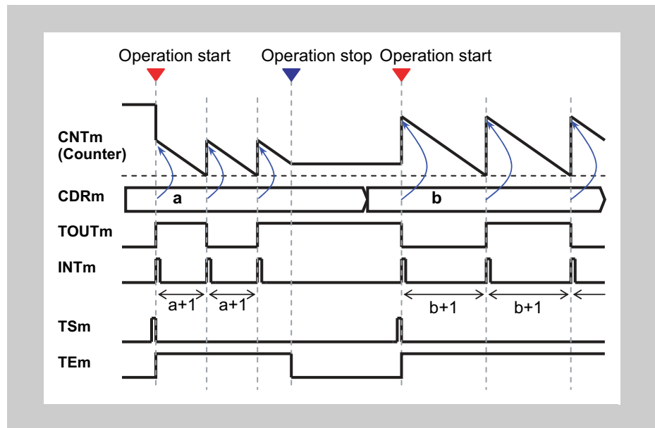
Figure 15-24 Operation stop and restart, \text{TAUJnCMORm.MD0} = 1
