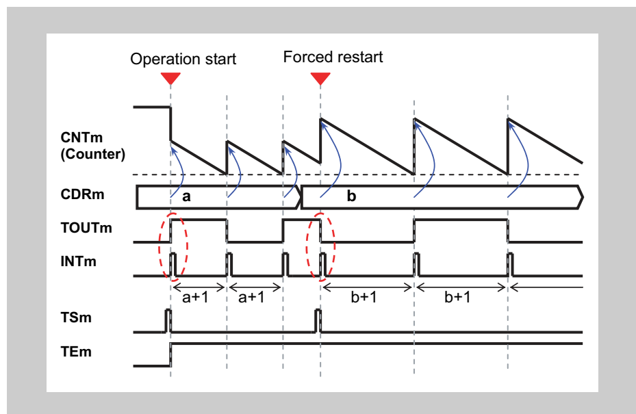
Figure 15-25 Forced restart operation, \text{TAUJnCMORm.MD0} = 1
