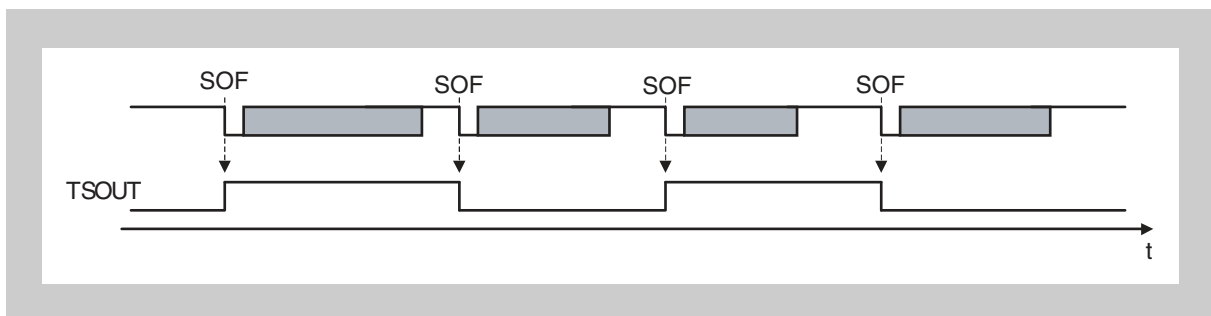
Figure 18-14 Timing diagram of capture signal TSOUT
