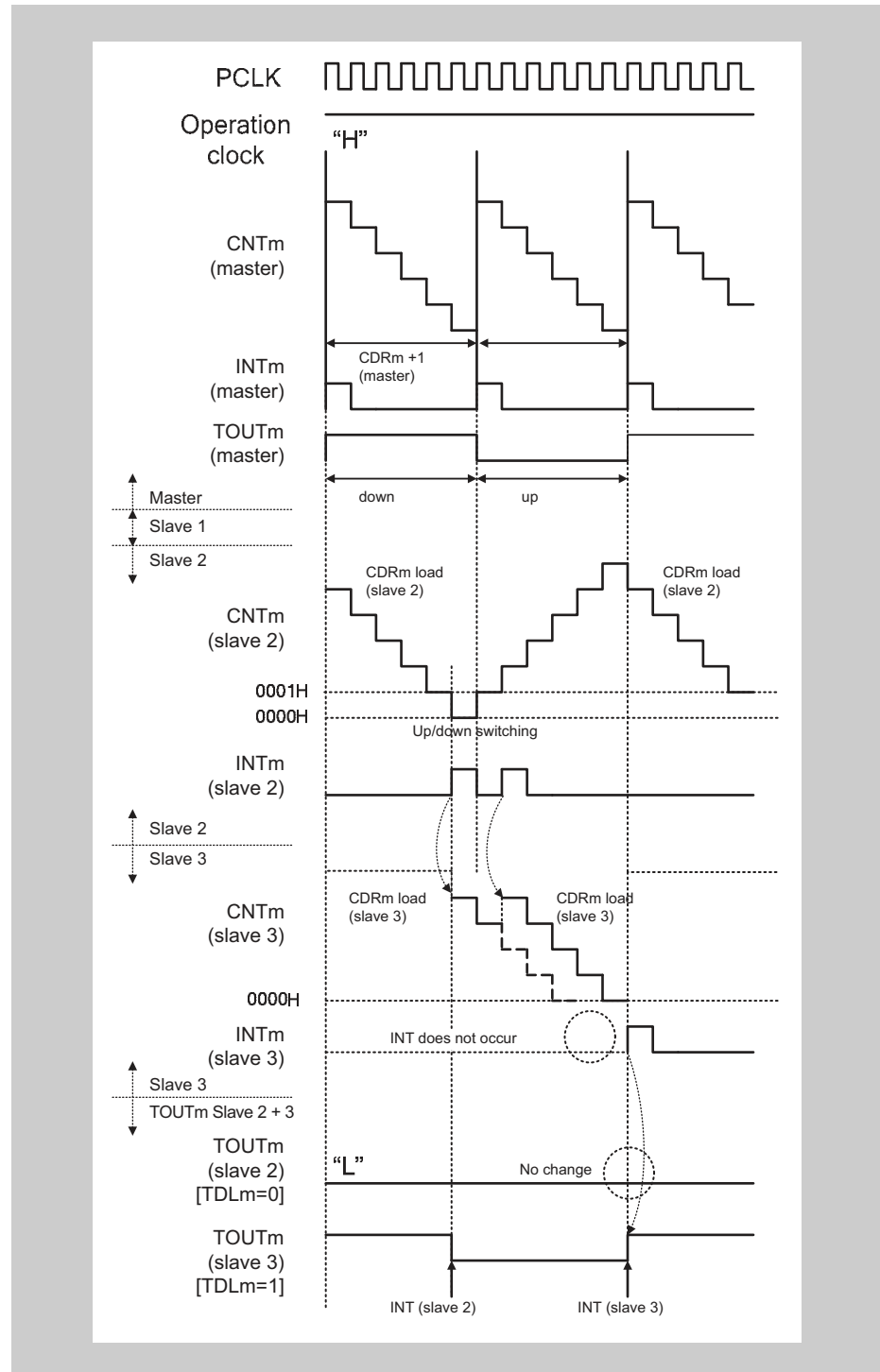
Figure 14-94 TAUBnCDRm (master) = 0005 H , TAUBnCDRm (slave 2) = 0005 H , TAUBnCDRm (slave 3) = 0004 H
