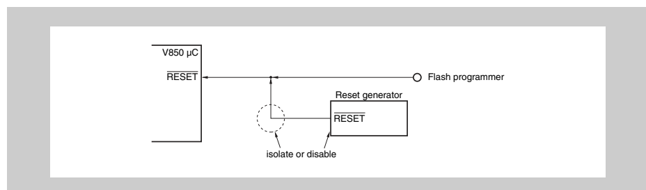
Figure 6-7 Potential conflict with \overline{\text{RESET}}
