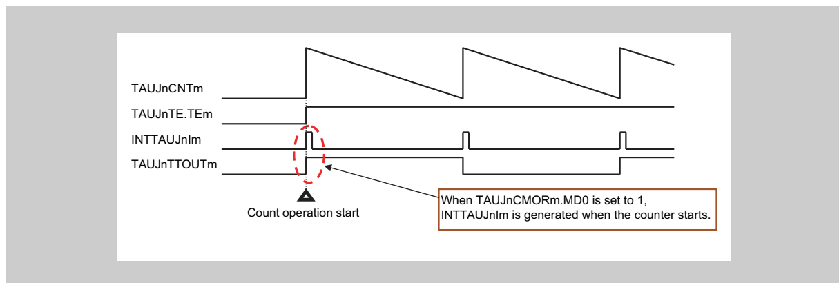
Figure 15-9 INTTAUJnIm generated when counter starts
