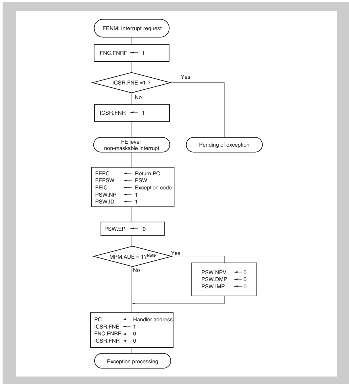
Figure 4-1 Processing upon occurrence of FENMI interrupt request
