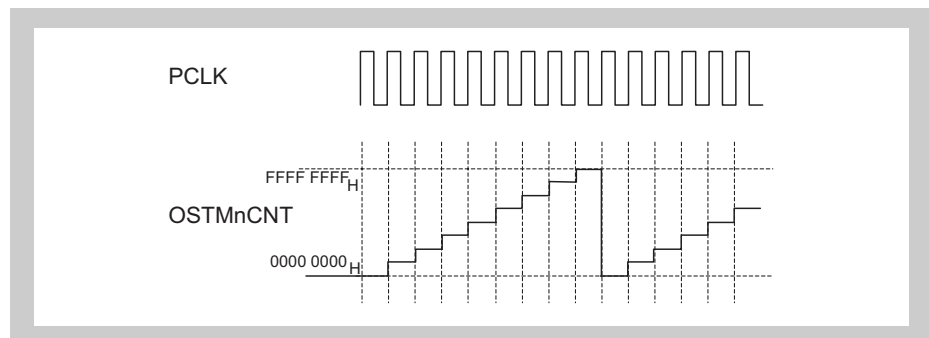
Figure 12-3 Counter operation
