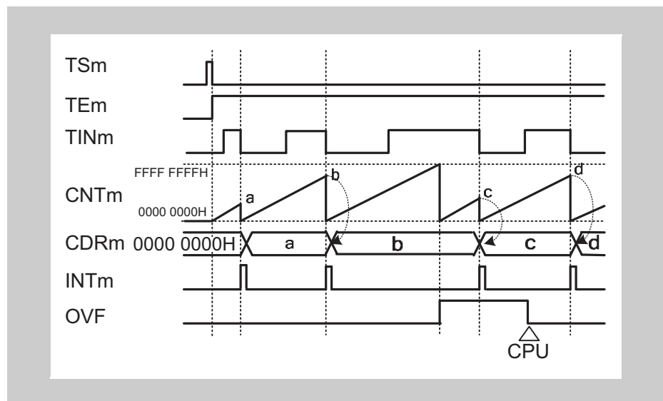
Figure 15-32 TAUJnCMORM.COS[1:0] = 01 B , TAUJnCMORM.MD0 = 0, TAUJnCMURm.TIS[1:0]=00 B
