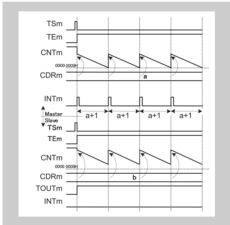
Figure 15-54 TAUJnCDRm (slave) \geq TAUJnCDRm (master) + 1, positive logic (TAUJnTOL.TOLm (slave) = 0)
