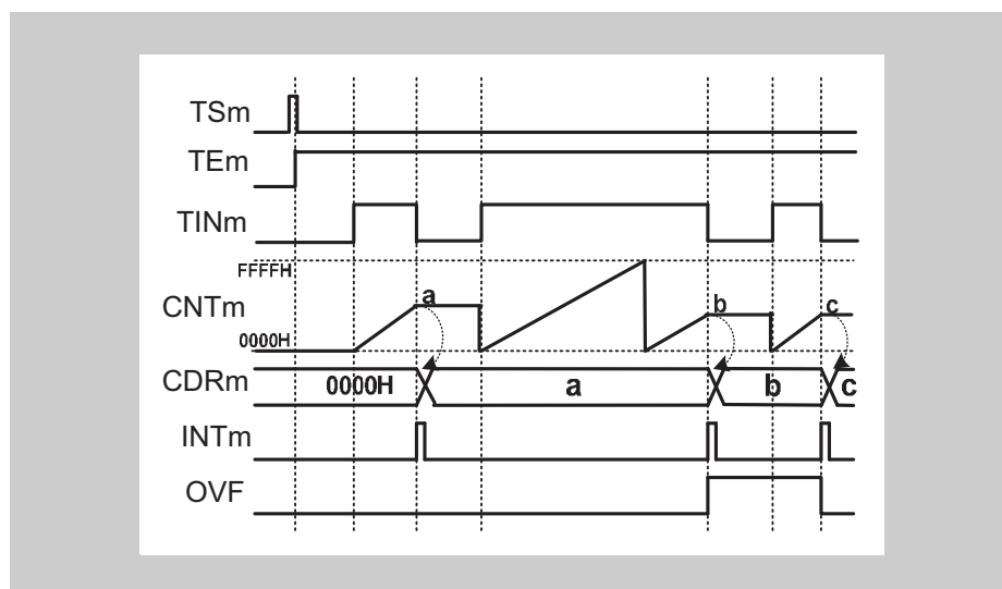
Figure 14-39 TAUBnCMORm.COS[1:0] = 00 B , TAUBnCMORm.MD0 = 0, TAUBnCMURm.TIS[1:0]=11 B
