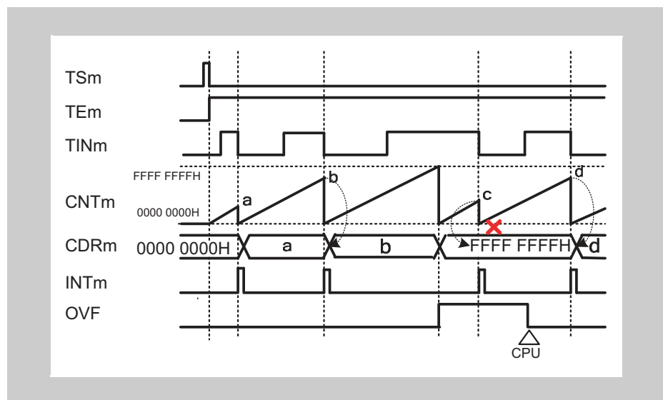
Figure 15-34 \text{TAUJnCMORM.COS}[1:0] = 11_{\text{B}} , \text{TAUJnCMORM.MD0} = 0 , \text{TAUJnCMURm.TIS}[1:0] = 00_{\text{B}}
