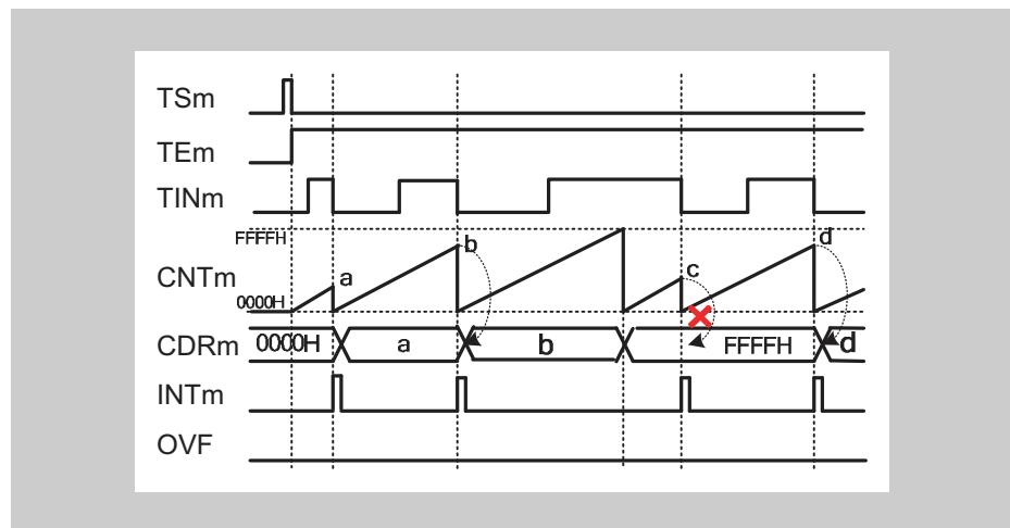
Figure 14-35 \text{TAUBnCMORm.COS}[1:0] = 10_{\text{B}} , \text{TAUBnCMORm.MD0} = 0 , \text{TAUBnCMURm.TIS}[1:0] = 00_{\text{B}}
