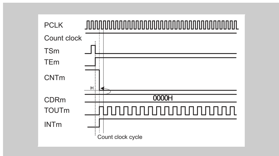
Figure 14-22 TAUBnCDRm = 0000 H , count clock = PCLK
