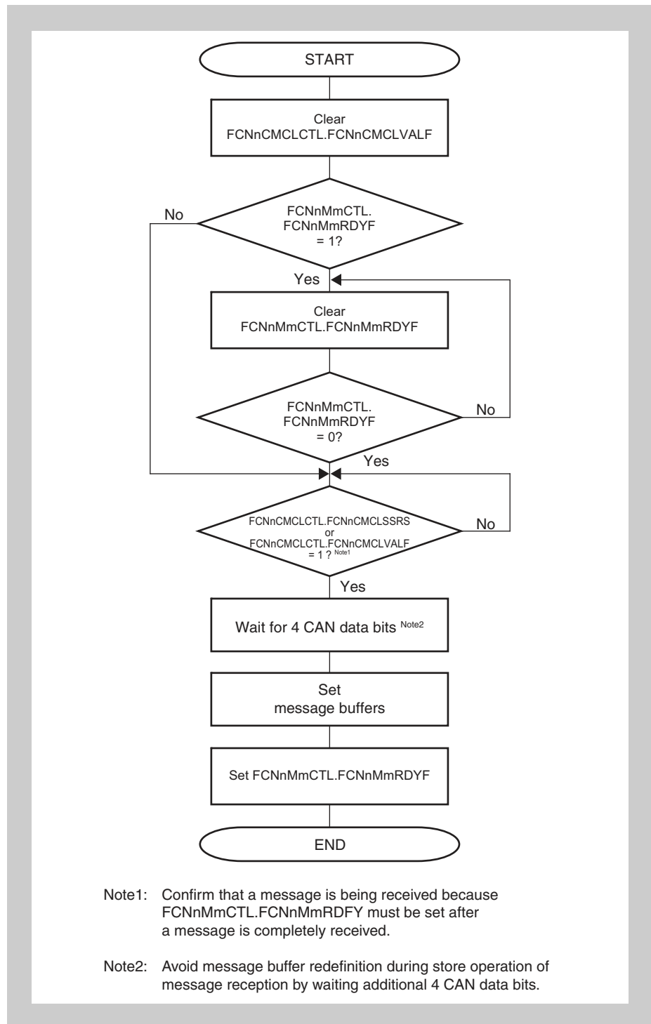
Figure 18-20 Message buffer redefinition during reception
