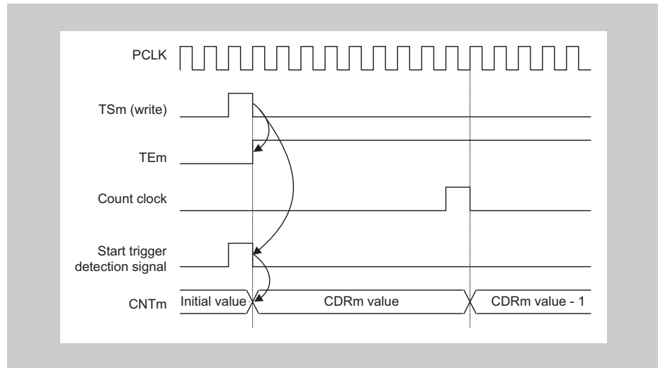
Figure 14-14 Start timing of Event Mode
