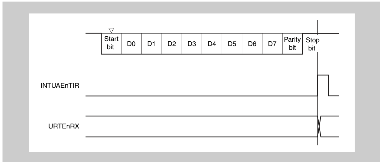
Figure 16-16 URTEEn reception
