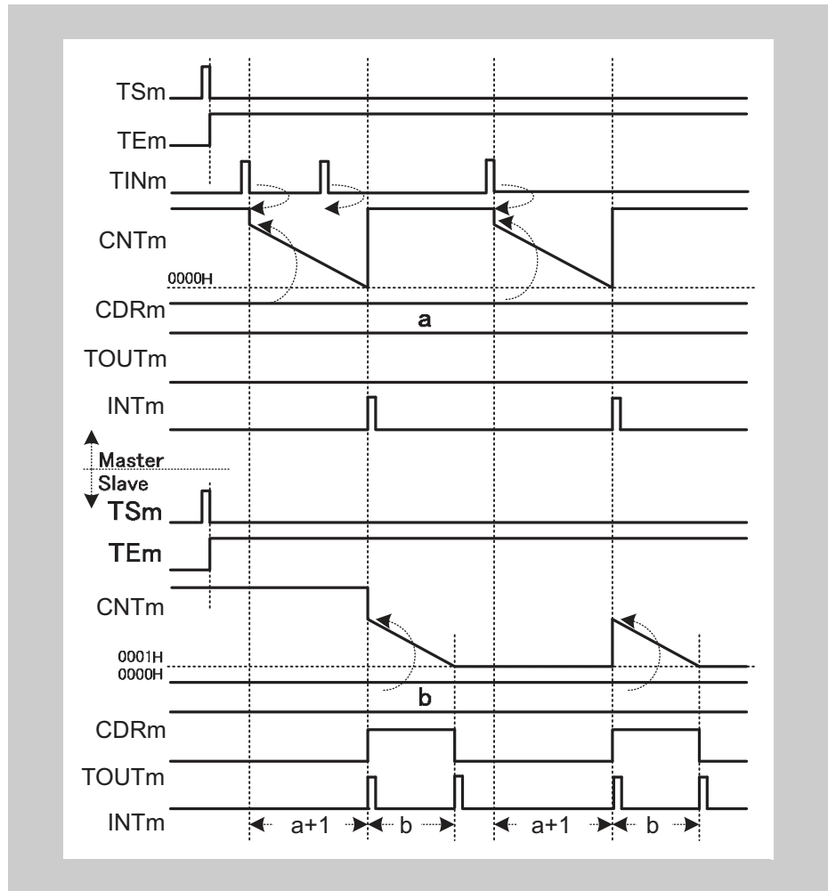
Figure 14-81 General timing diagram for One-Shot Pulse Output Function
