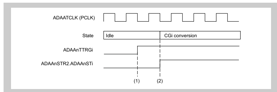
Figure 22-10 Hardware start trigger timing
