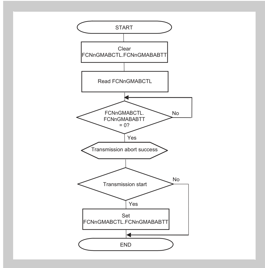
Figure 18-31 ABT transmission request abort processing (normal operation mode with ABT) with transmit abort interrupt flag
