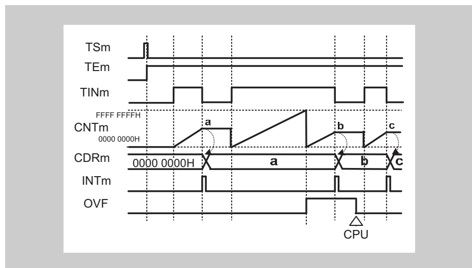
Figure 15-38 \text{TAUJnCMORM.COS}[1:0] = 01_{\text{B}} , \text{TAUJnCMORM.MD0} = 0 , \text{TAUJnCMURm.TIS}[1:0] = 11_{\text{B}}
