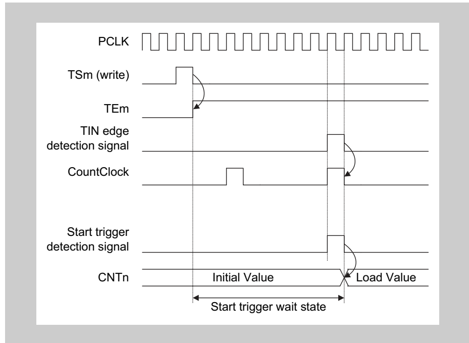
Start timing of all other operating modes
