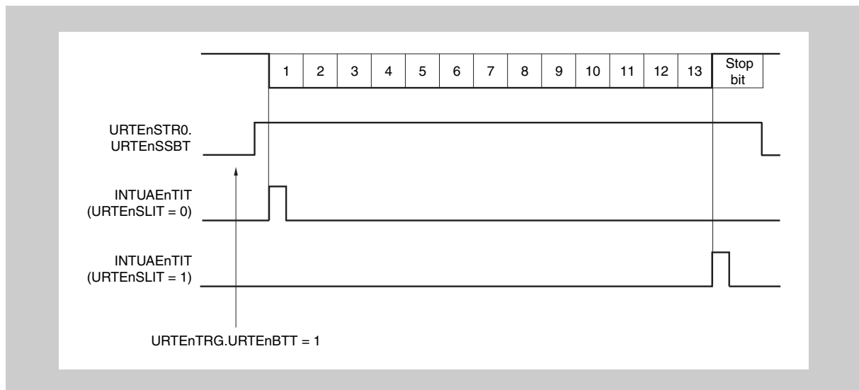
Figure 16-8 BF transmission
