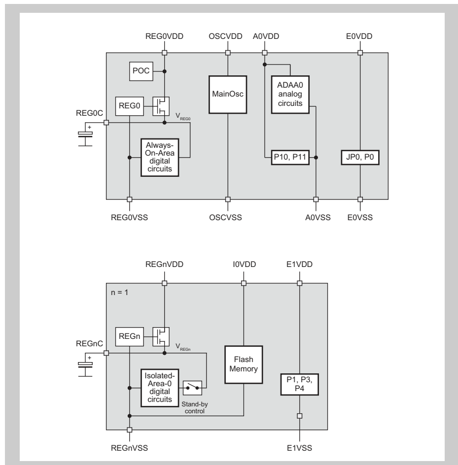
Figure 24-3 V850E2S/FG4-L power supply scheme
