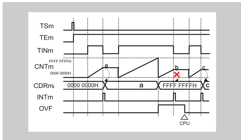
Figure 15-40 \text{TAUJnCMORM.COS}[1:0] = 11_{\text{B}} , \text{TAUJnCMORM.MD0} = 0 , \text{TAUJnCMURM.TIS}[1:0] = 11_{\text{B}}
