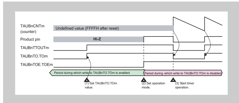
Figure 14-10 General procedure for specifying a TAUBnTTOUTm channel output mode
