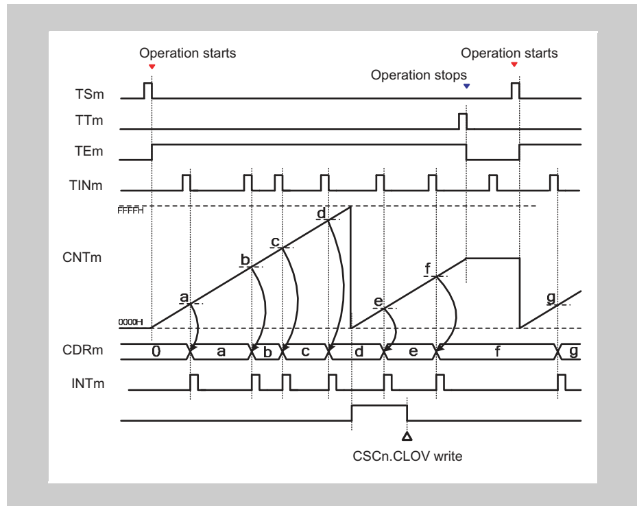
Figure 14-68 Operation stop and restart, TAUBnCMORm.MD0 = 0, TAUBnCMURm.TIS[1:0] = 00
