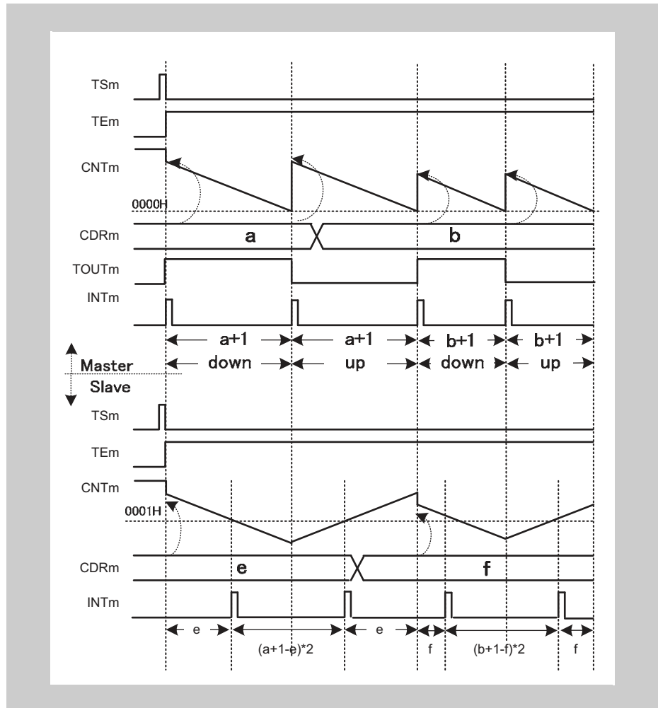
Figure 14-99 General timing diagram for AD Conversion Trigger Output Function Type 2
