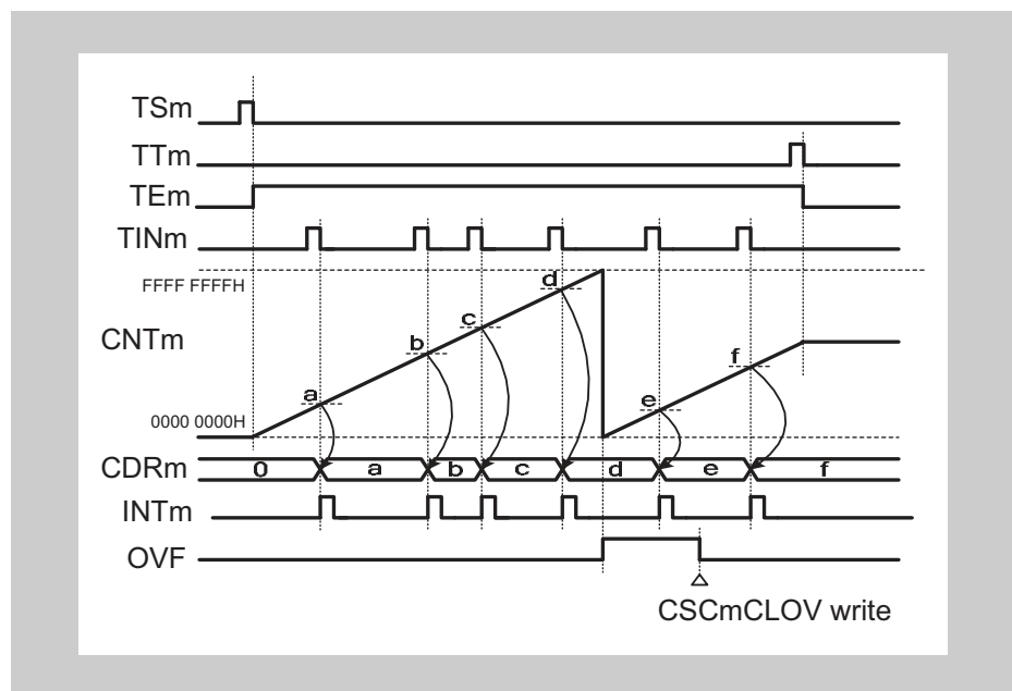
Figure 15-49 General timing diagram for TAUJnTTINm Input Position Detection Function
