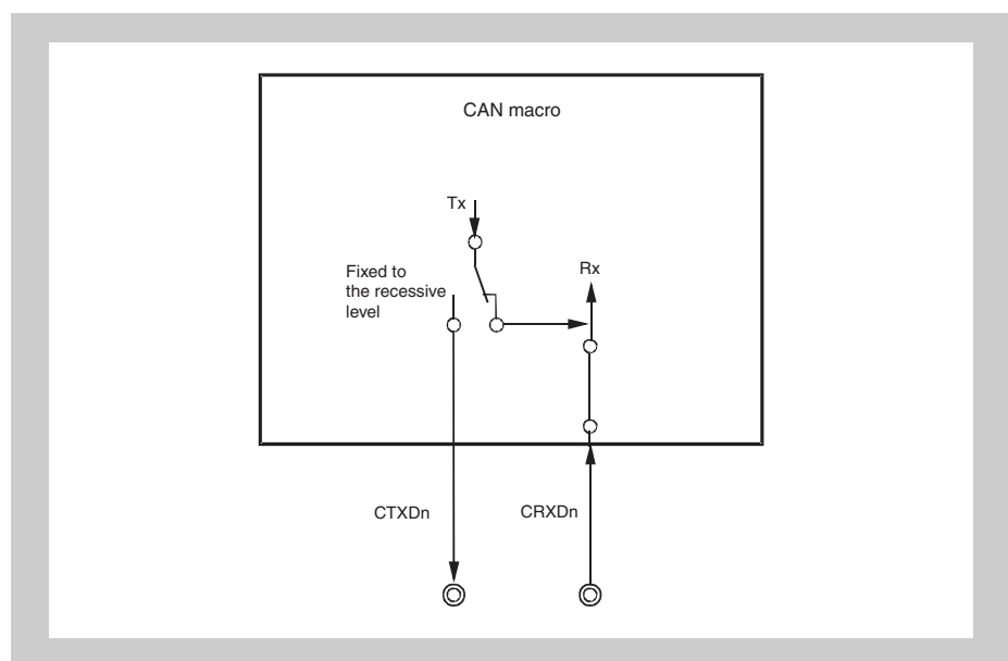
Figure 18-12 CAN Controller terminal connection in receive-only mode
