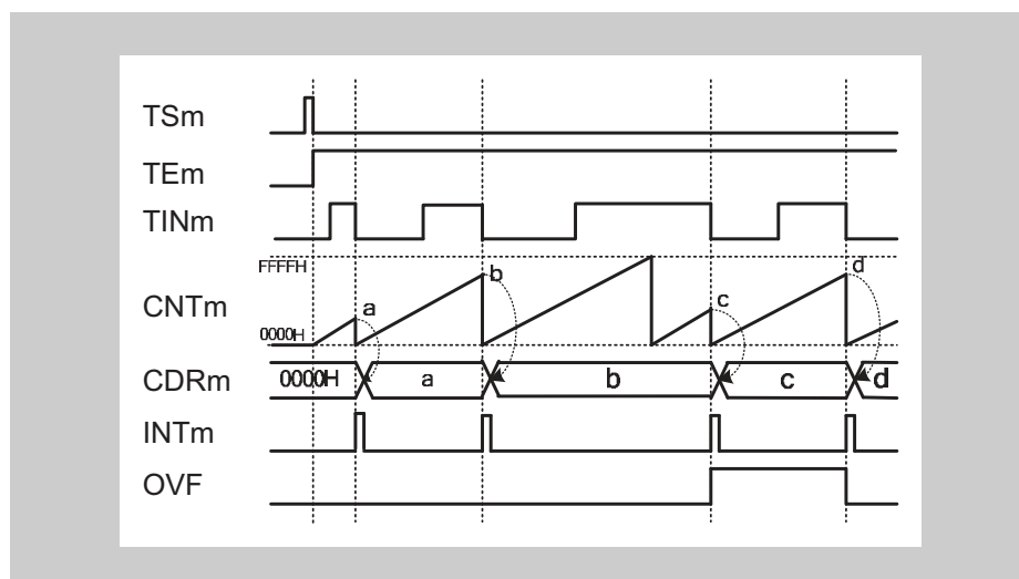
Figure 14-33 TAUBnCMORm.COS[1:0] = 00_B , TAUBnCMORm.MD0 = 0 , TAUBnCMURm.TIS[1:0] = 00_B
