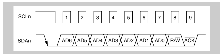
Figure 20-8 Acknowledge ( \overline{\text{ACK}} )
