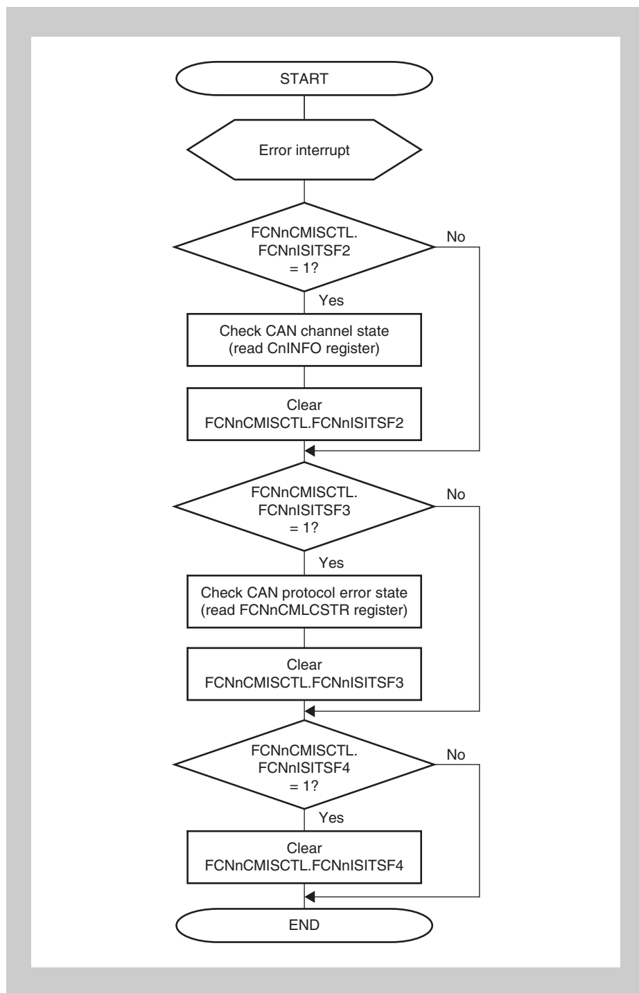
Figure 18-43 Error handling
