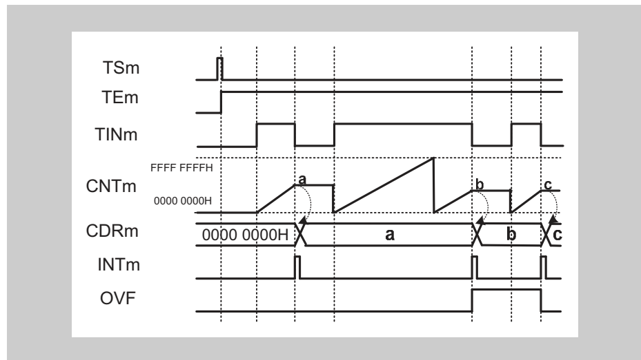
Figure 15-37 \text{TAUJnCMORM.COS}[1:0] = 00_{\text{B}} , \text{TAUJnCMORM.MD0} = 0 , \text{TAUJnCMURm.TIS}[1:0] = 11_{\text{B}}
