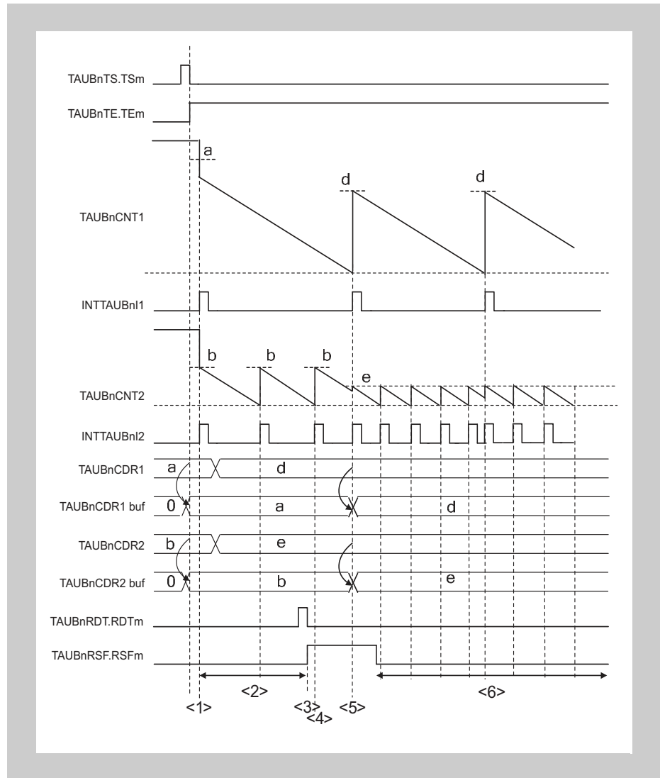
Figure 14-55 General timing diagram for Simultaneous Rewrite Trigger Generation Function Type 1
