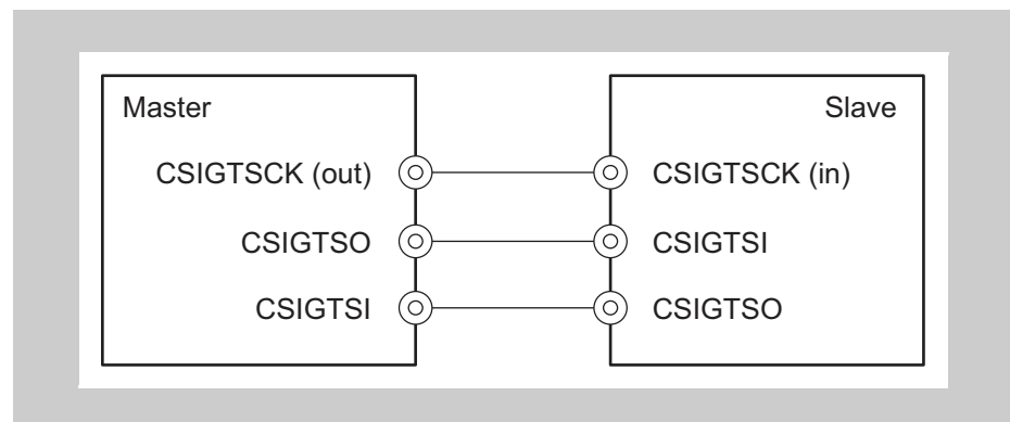
Figure 19-5 Simple master/slave connection
