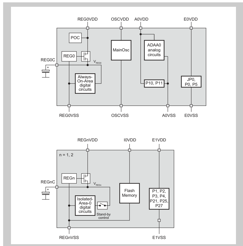
Figure 24-4 V850E2S/FJ4-L power supply scheme
