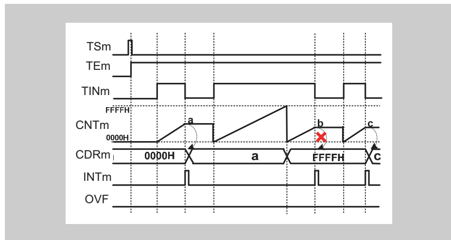
Figure 14-41 \text{TAUBnCMORm.COS}[1:0] = 10_{\text{B}} , \text{TAUBnCMORm.MD0} = 0 , \text{TAUBnCMURm.TIS}[1:0] = 11_{\text{B}}
