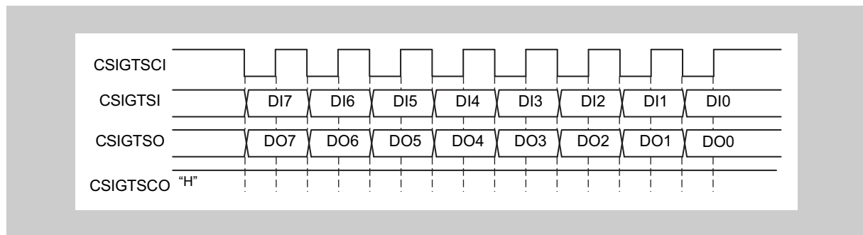
Figure 19-4 Transmit/receive in slave mode
