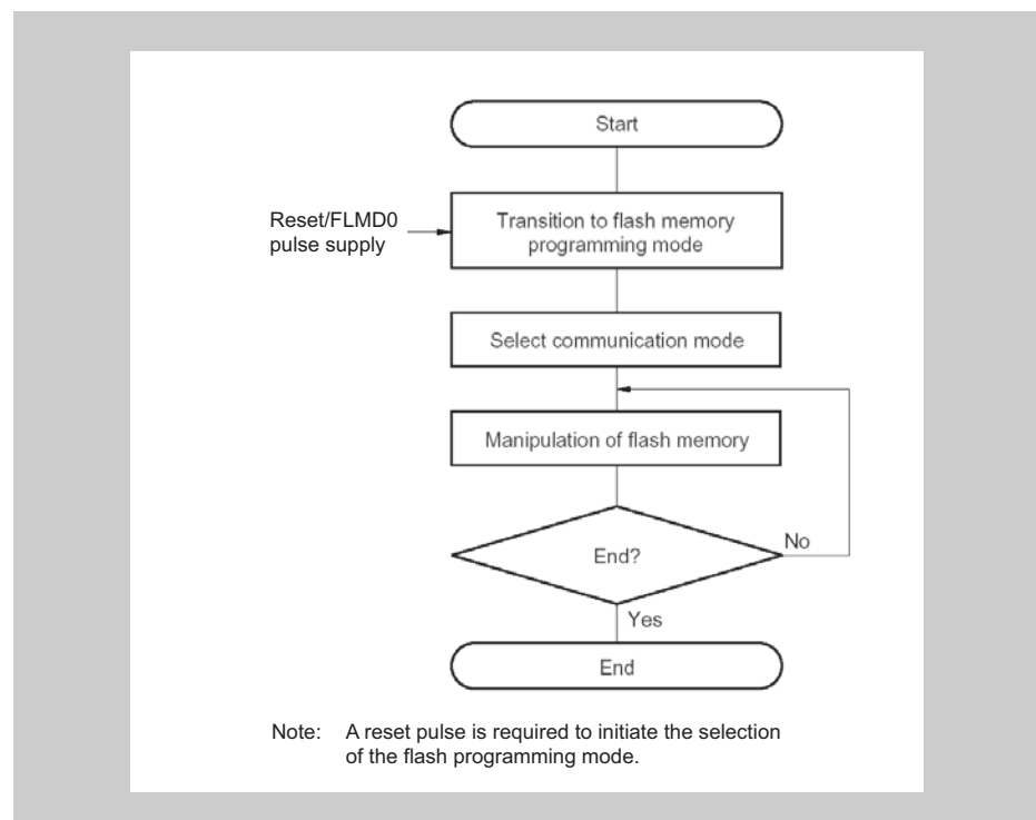
Figure 6-4 Flash memory programming procedure
