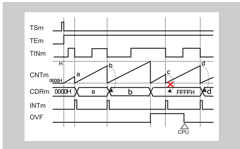
Figure 14-36 \text{TAUBnCMORm.COS}[1:0] = 11_{\text{B}} , \text{TAUBnCMORm.MD0} = 0 , \text{TAUBnCMURm.TIS}[1:0] = 00_{\text{B}}
