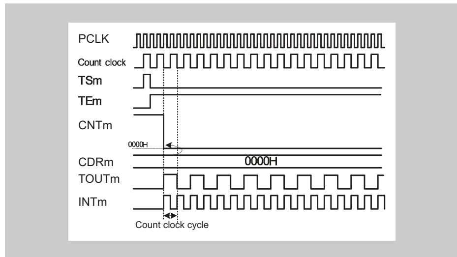
Figure 14-21 TAUBnCDRm = 0000 H , count clock = PCLK/2
