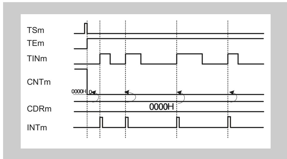
Figure 14-58 TAUBnCDRm = 0000 H , TAUBnCMURm.TIS[1:0] = 01
