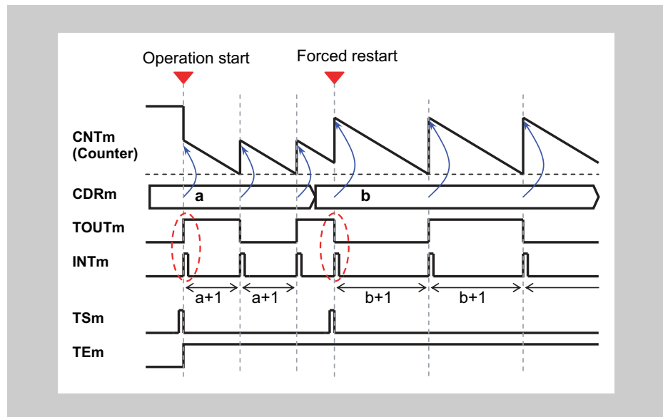
Figure 14-24 Forced restart operation, TAUBnCMORm.MD0 = 1
