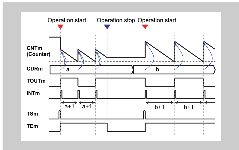
Figure 14-23 Operation stop and restart, TAUBnCMORm.MD0 = 1
