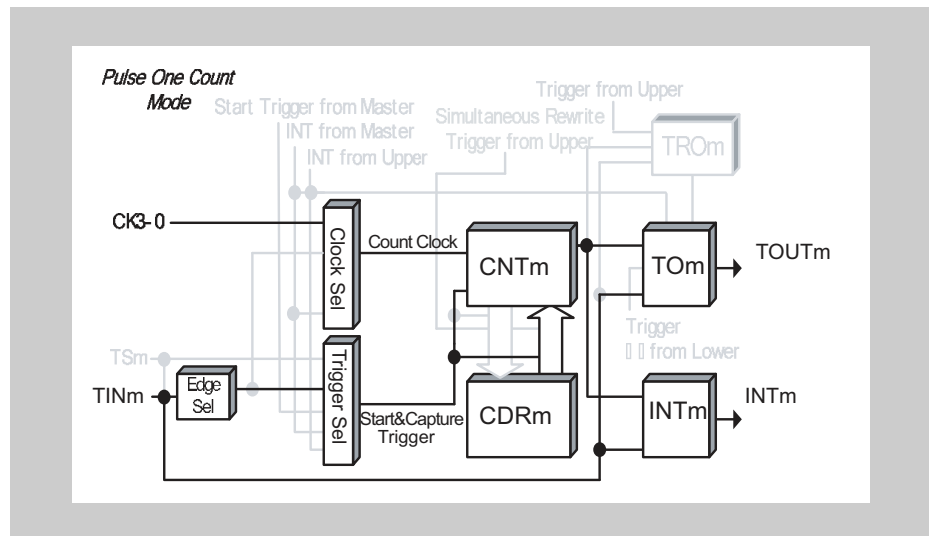
Figure 14-29 Block diagram for One-Pulse Output Function
