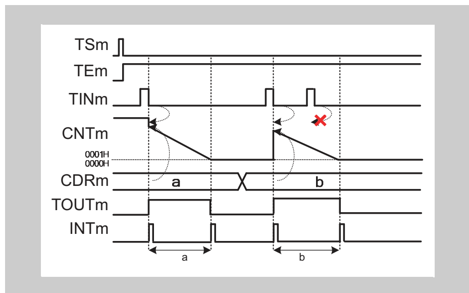
Figure 14-30 General timing diagram for One-Pulse Output Function
