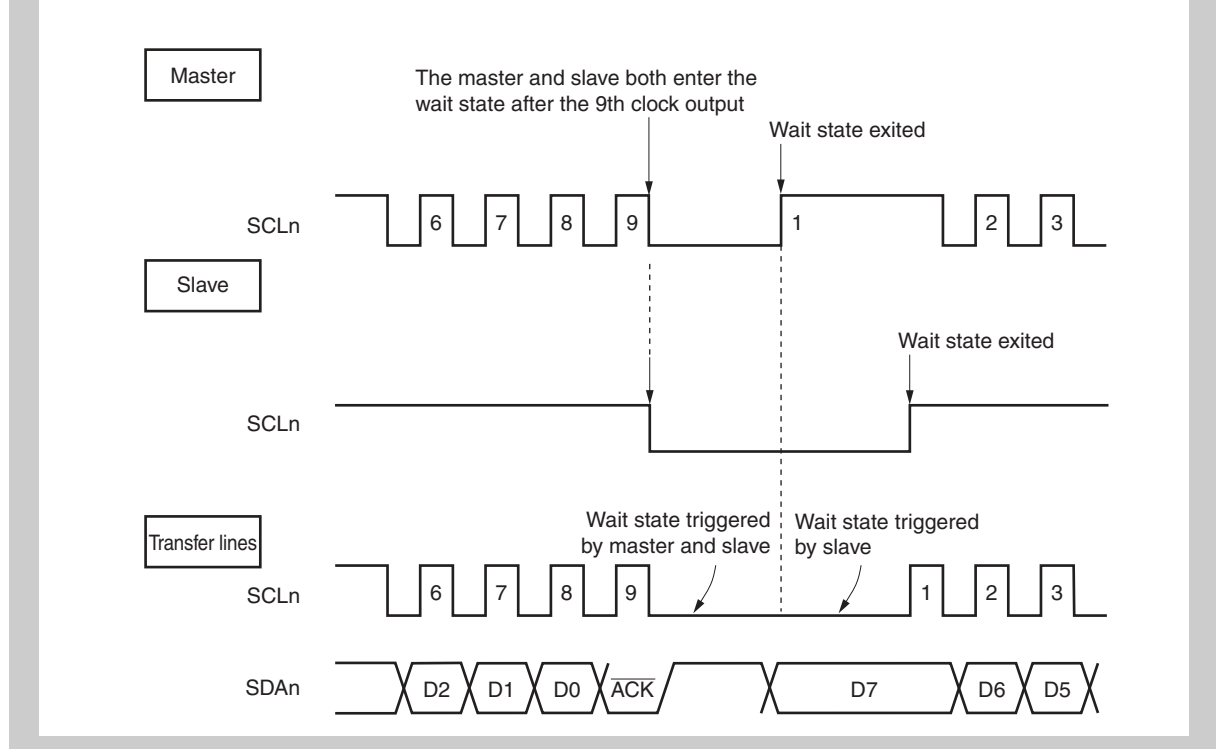
Figure 20-10 Wait state (2/2)
