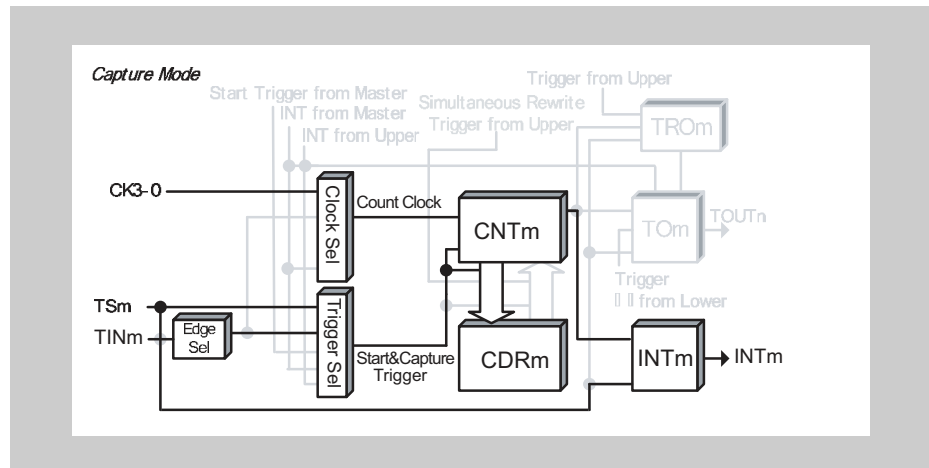
Figure 15-29 Block diagram for TAUJnTTINm Input Pulse Interval Measurement Function
