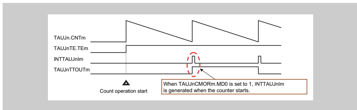
Figure 15-10 INTTAUJnIm not generated when counter starts
