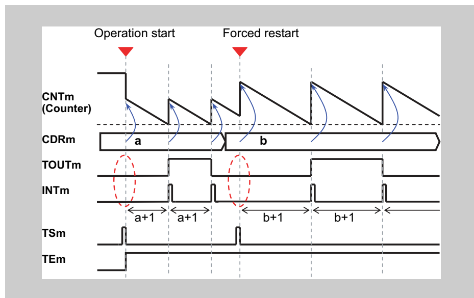
Figure 14-25 Forced restart operation, TAUBnCMORm.MD0 = 0
