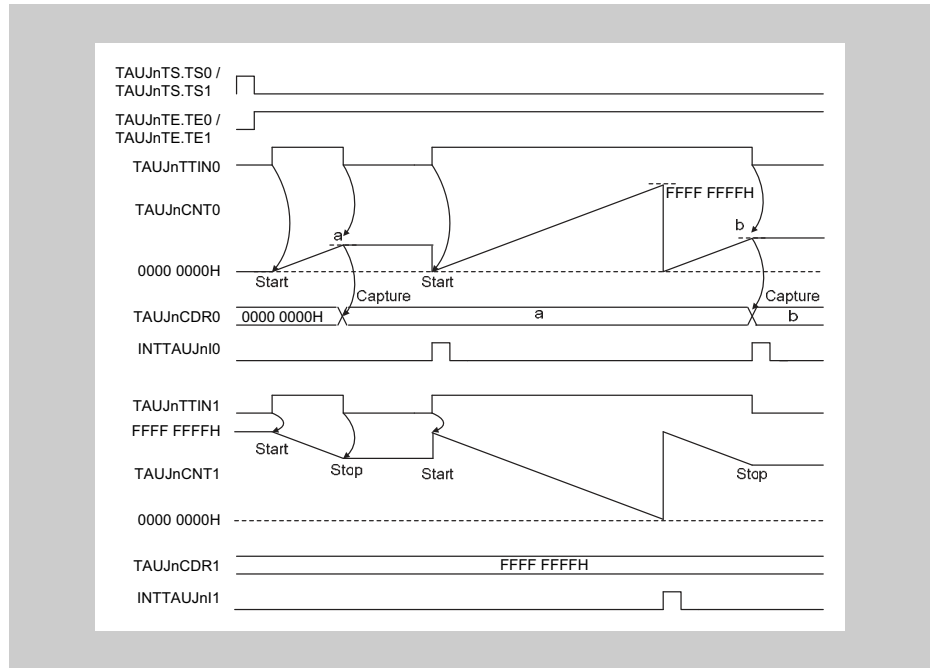
Figure 15-14 Interrupt generation via combination of Capture and One Count Mode and One Count Mode
