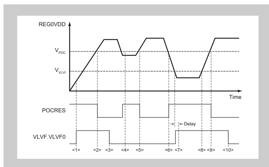
Figure 11-4 VLVI timing
