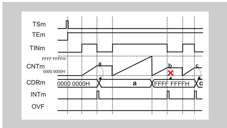
Figure 15-39 \text{TAUJnCMORM.COS}[1:0] = 10_{\text{B}} , \text{TAUJnCMORM.MD0} = 0 , \text{TAUJnCMURM.TIS}[1:0] = 11_{\text{B}}
