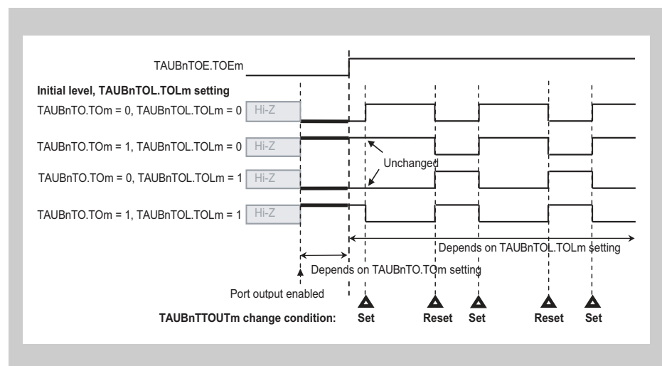
Figure 14-11 General change of the TAUBnTTOUTm output
