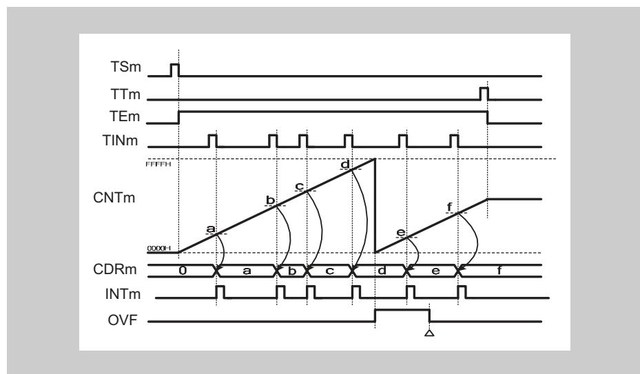
Figure 14-67 General timing diagram for TAUBnTTINm Input Position Detection Function
