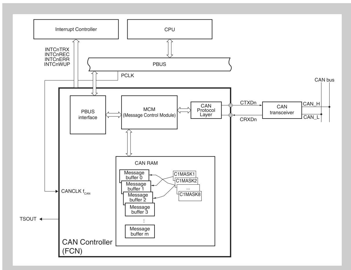
Figure 18-3 Block diagram of the CAN Controller
