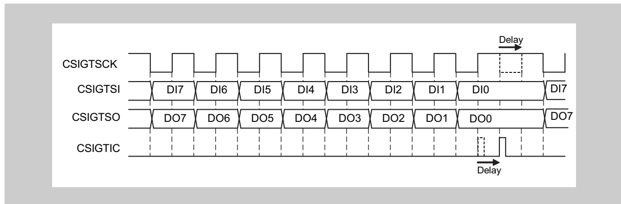
Figure 19-13 Interrupt delay function (CSIGnCTL1.CSIGnSIT = 1)
