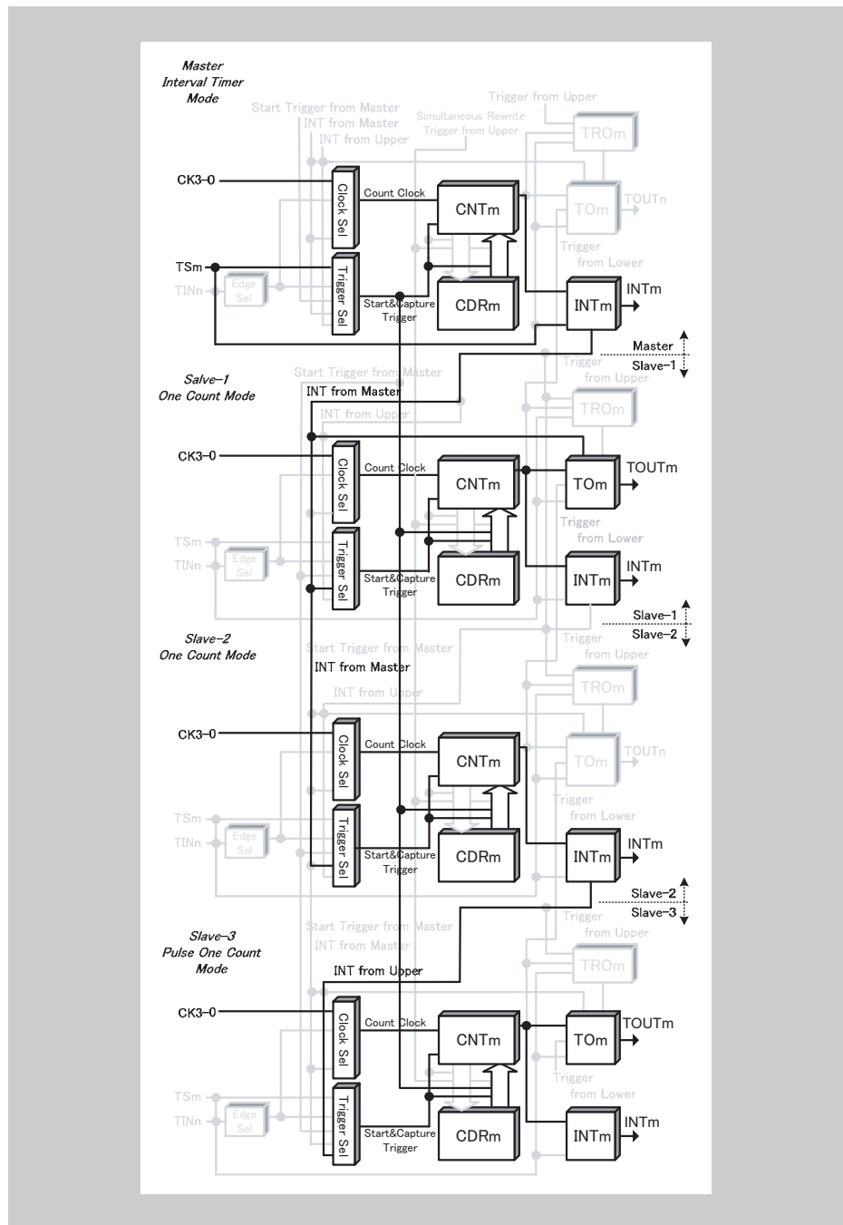
Figure 14-74 Block diagram for Delay Pulse Output Function
