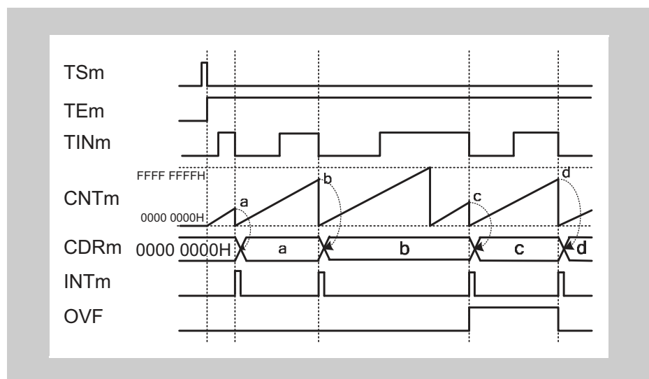
Figure 15-30 General timing diagram for TAUJnTTINm Input Pulse Interval Measurement Function
