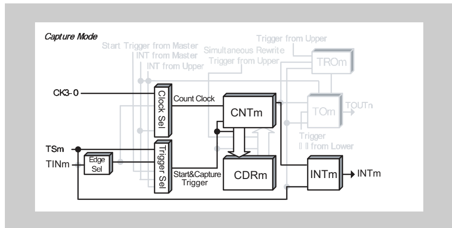
Figure 14-31 Block diagram for \text{TAUBnTTINm} Input Pulse Interval Measurement Function
