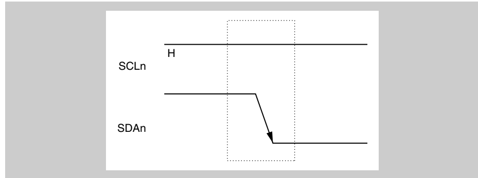
Figure 20-5 Start condition
