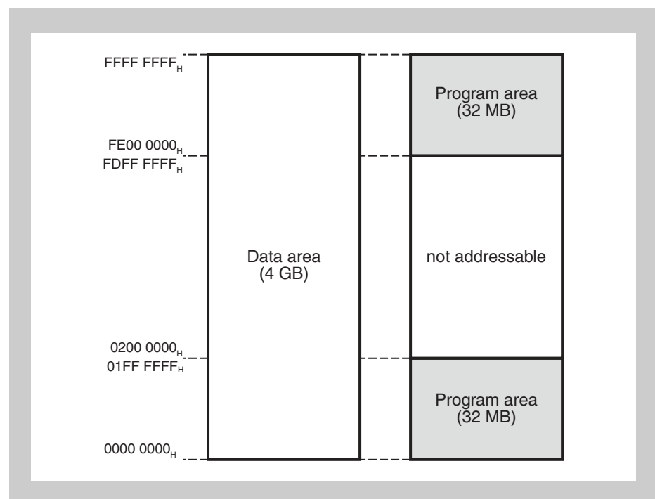
Figure 3-9 CPU address space
