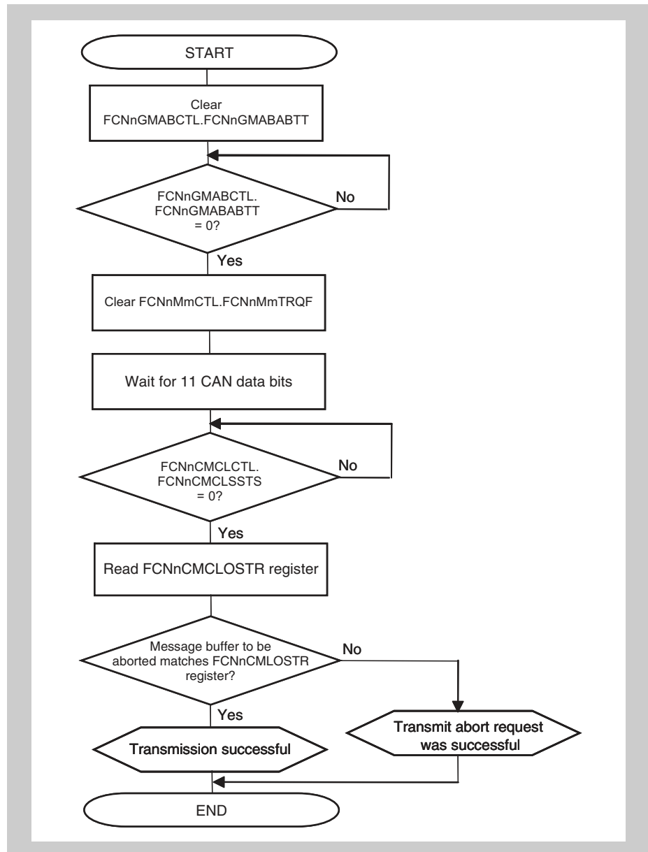
Figure 18-28 Transmission abort processing (normal operation mode with ABT) - Repeat option for aborted message
