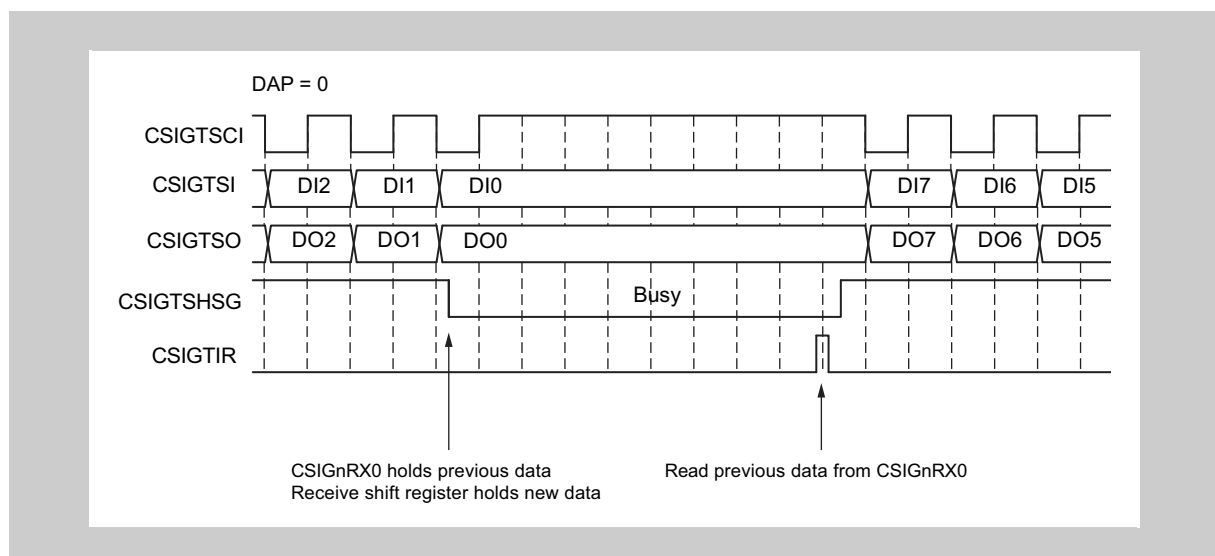
Figure 19-17 Ready/busy signal from slave (CSIGNCFG0.CSIGNDAP = 0)
