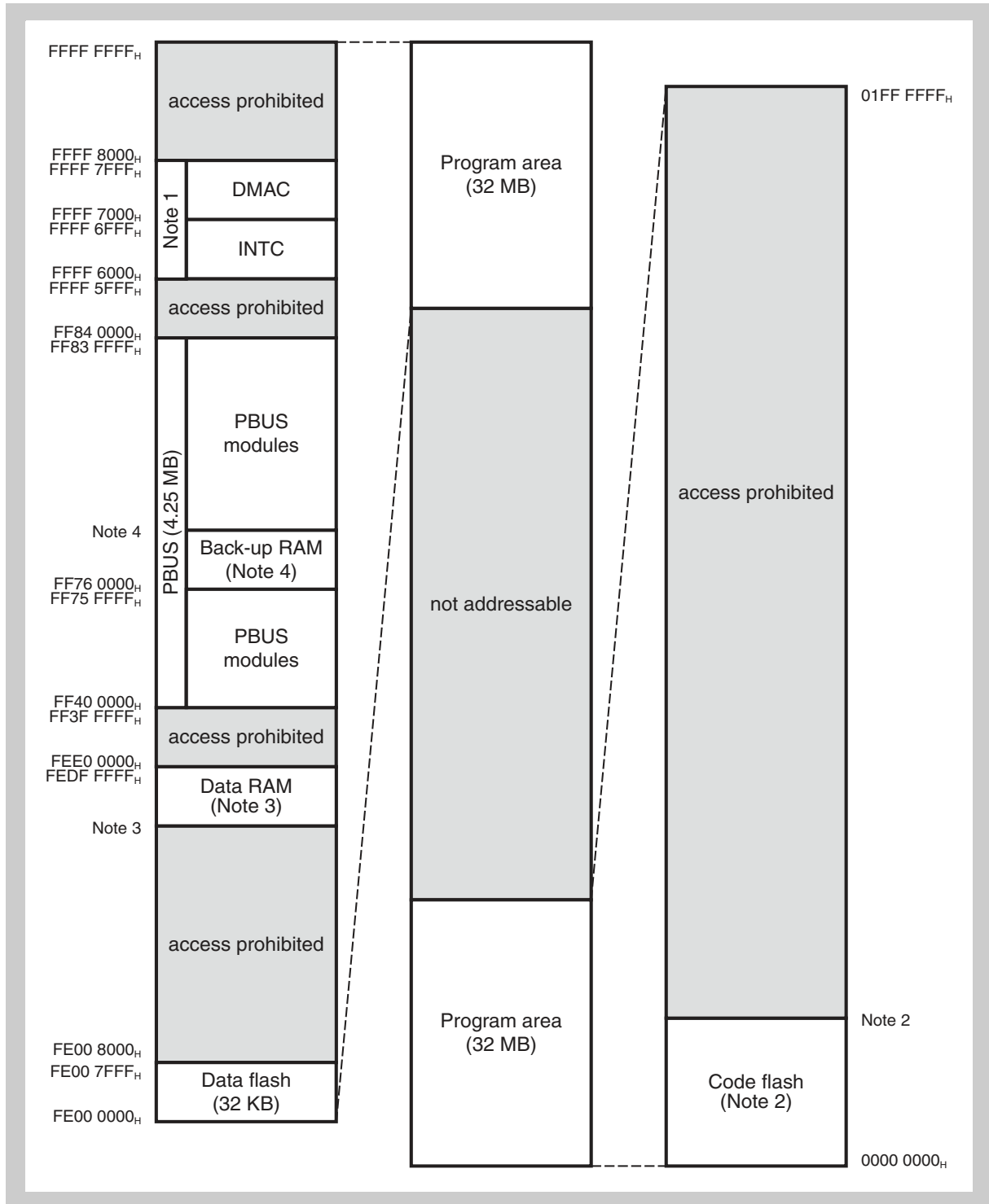
Figure 3-12 Memory map
