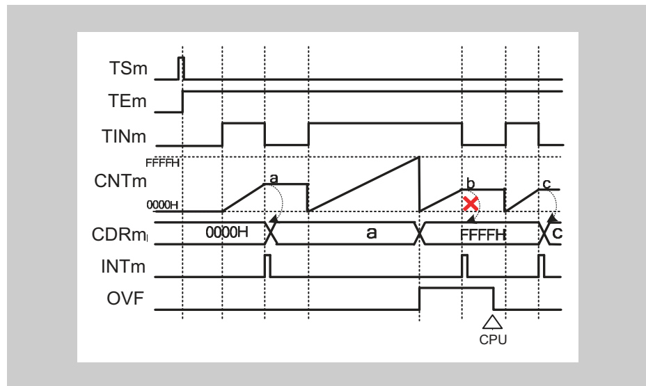
Figure 14-42 \text{TAUBnCMORm.COS}[1:0] = 11_{\text{B}} , \text{TAUBnCMORm.MD0} = 0 , \text{TAUBnCMURm.TIS}[1:0] = 11_{\text{B}}
