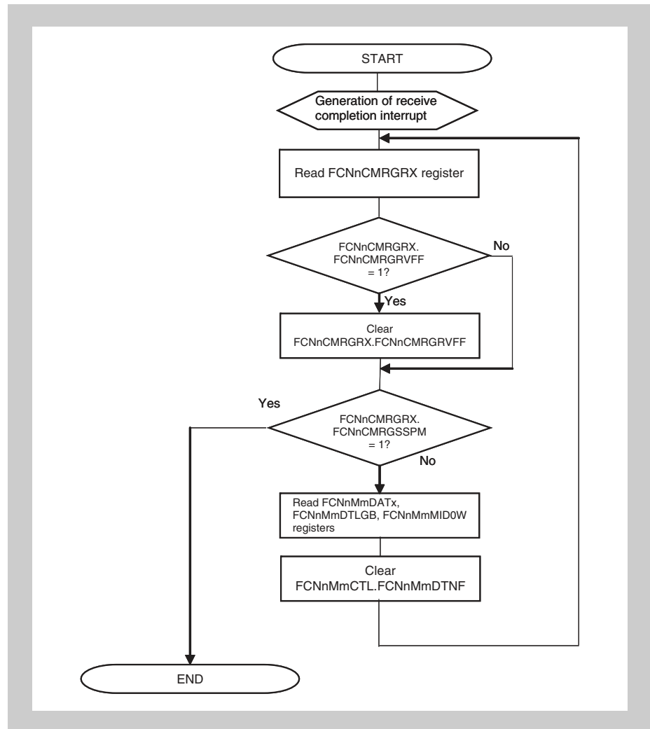
Figure 18-36 Reception via interrupt (using FCNnCMRGRX register), alternative way
