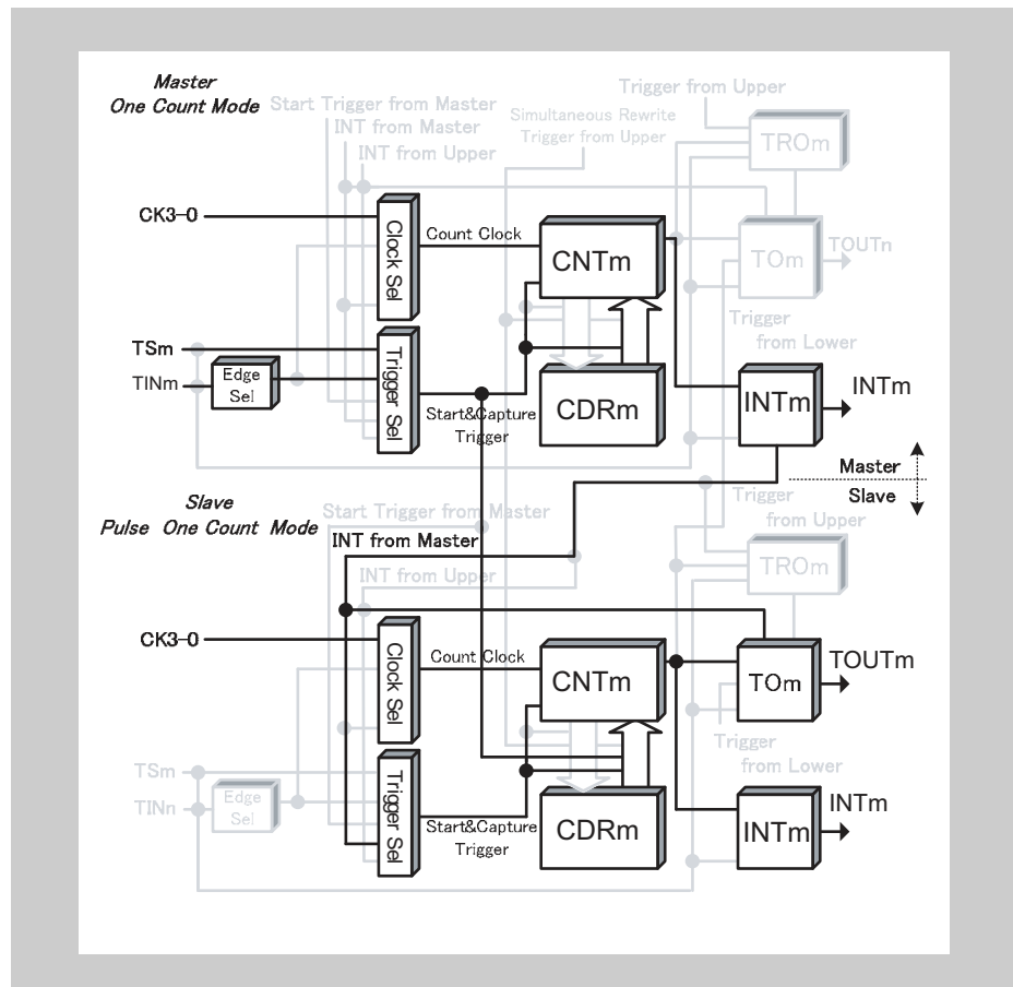
Figure 14-80 Block diagram for One-Shot Pulse Output Function
