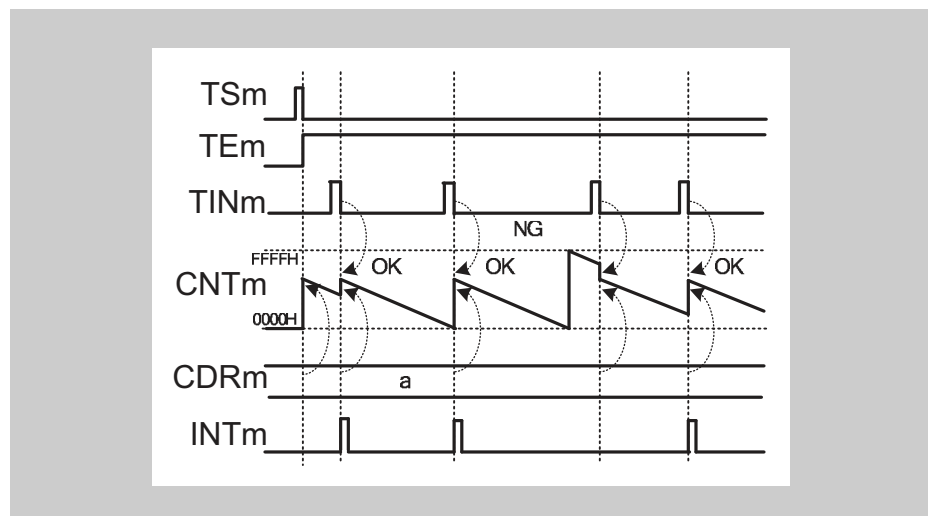
Figure 14-51 General timing diagram for TAUBnTTINm Input Pulse Interval Judgment Function
