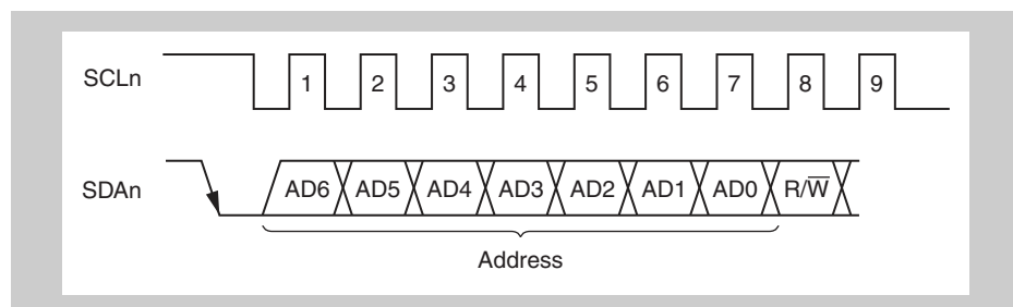
Figure 20-6 Addresses
