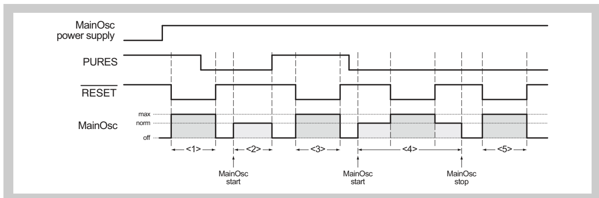
Figure 11-6 MainOsc behaviour during \overline{\text{RESET}}
