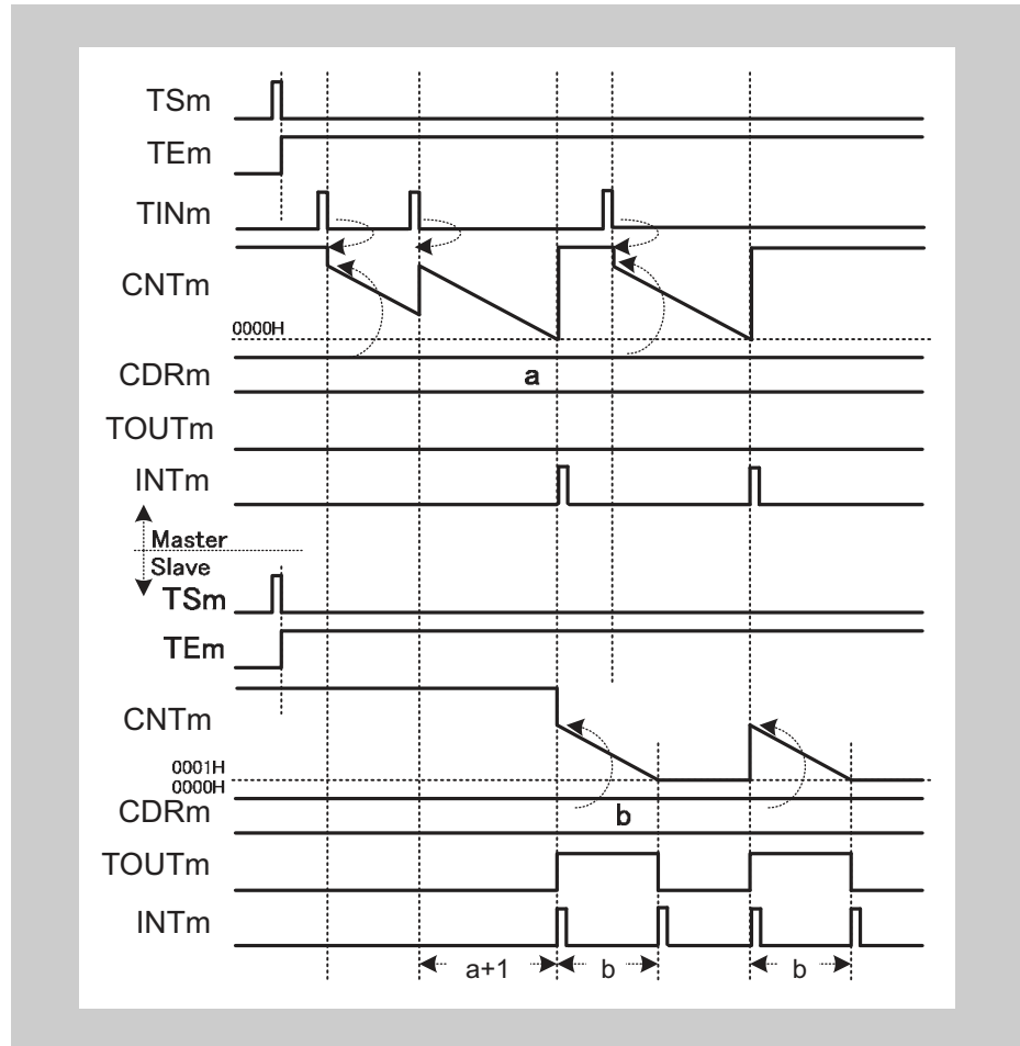
Figure 14-84 TAUBnCMORm.MD0 = 1
