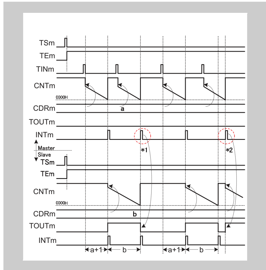
Figure 14-85 Interval of TAUBnTTINm ≤ delay time + pulse width + 1
