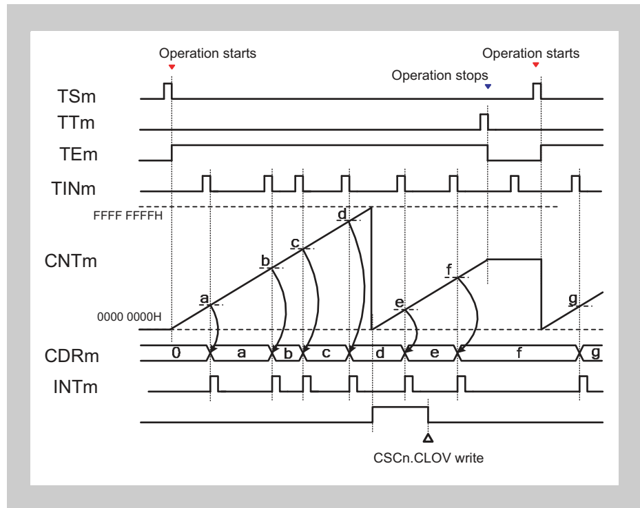
Figure 15-50 Operation stop and restart, TAUJnCMORM.MD0 = 0, TAUJnCMURm.TIS[1:0] = 00
