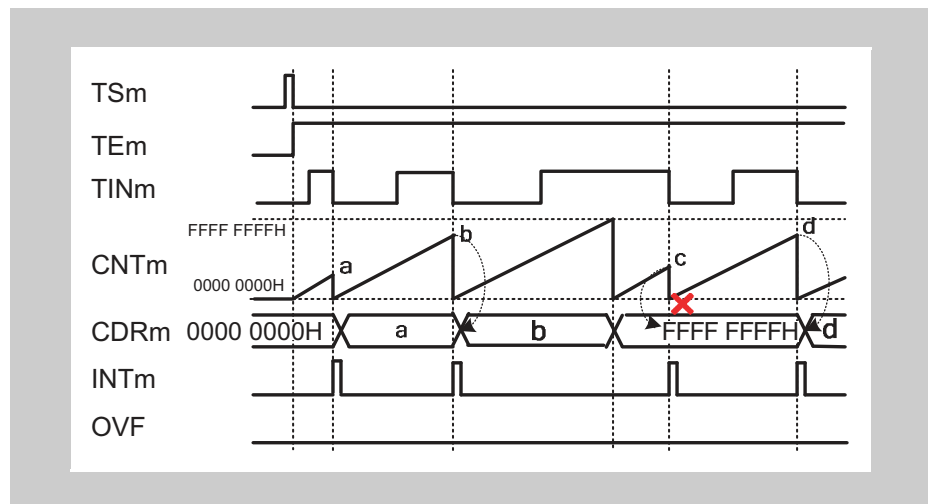
Figure 15-33 \text{TAUJnCMORM.COS}[1:0] = 10_{\text{B}} , \text{TAUJnCMORM.MD0} = 0 , \text{TAUJnCMURm.TIS}[1:0] = 00_{\text{B}}
