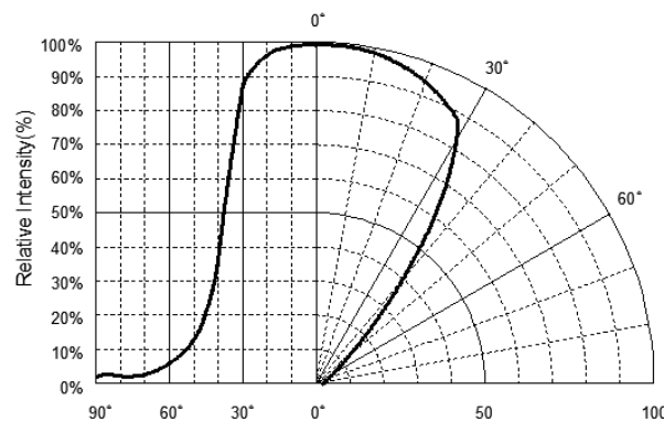
Fig 2. Radiation Characteristics
