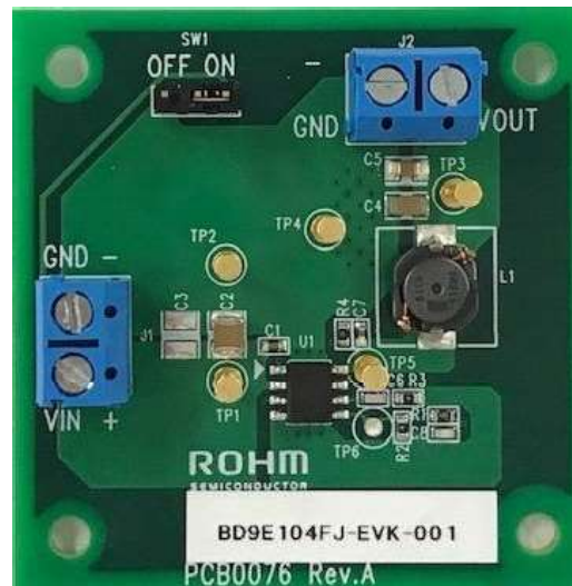
Figure 1. BD9E104FJ-EVK-001(Top View)
