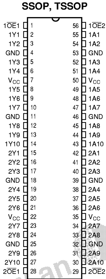
Figure 2. Pin Configuration (All Pins Top View)
