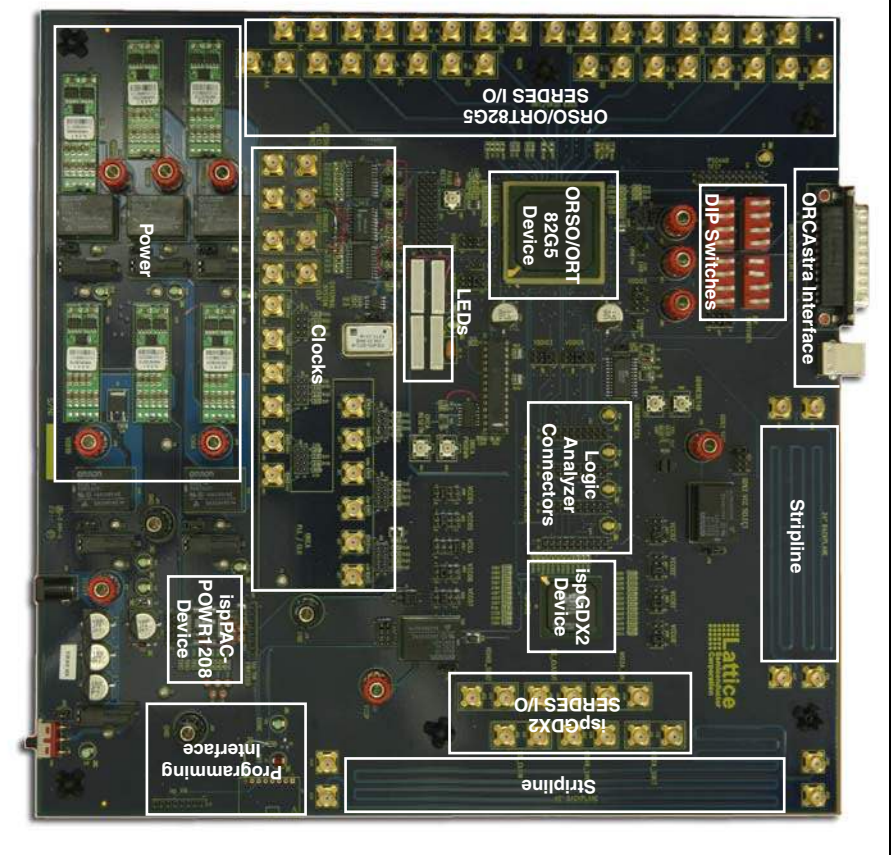
Figure 1. Lattice High-Speed SERDS Briccase Board
