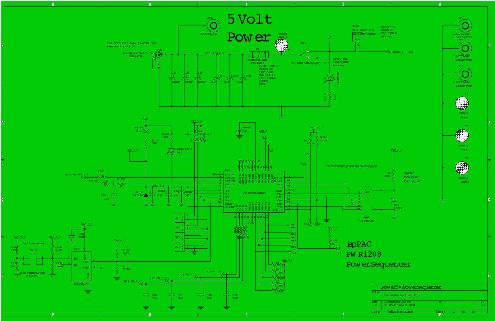
Figure 14. Lattice High-Speed SERDES Briefcase Board Schematic
