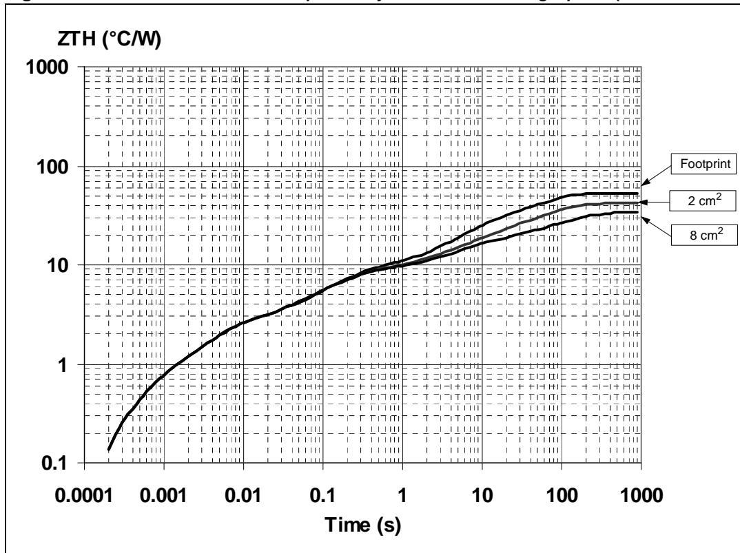
Figure 30. PowerSSO-24 thermal impedance junction ambient single pulse (one channel on)
