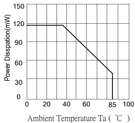
Ambient Temperature vs. Total Power Dissipation
