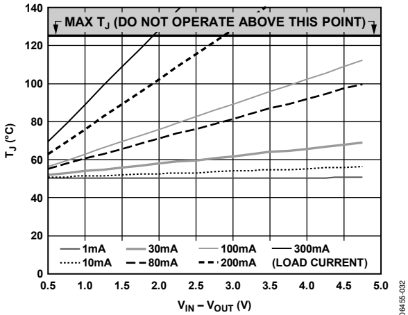
Figure 36. 500 mm 2 of PCB Copper, T A = 50°C
