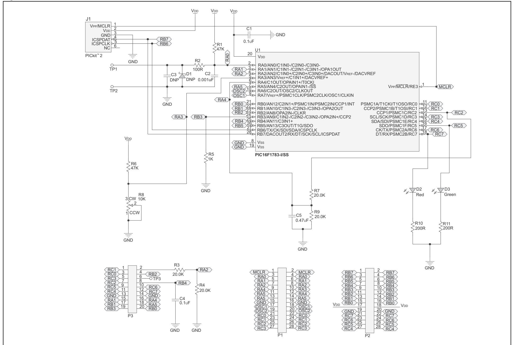
Figure 2: F1 PSMC 28-Pin Evaluation Platform Schematic
