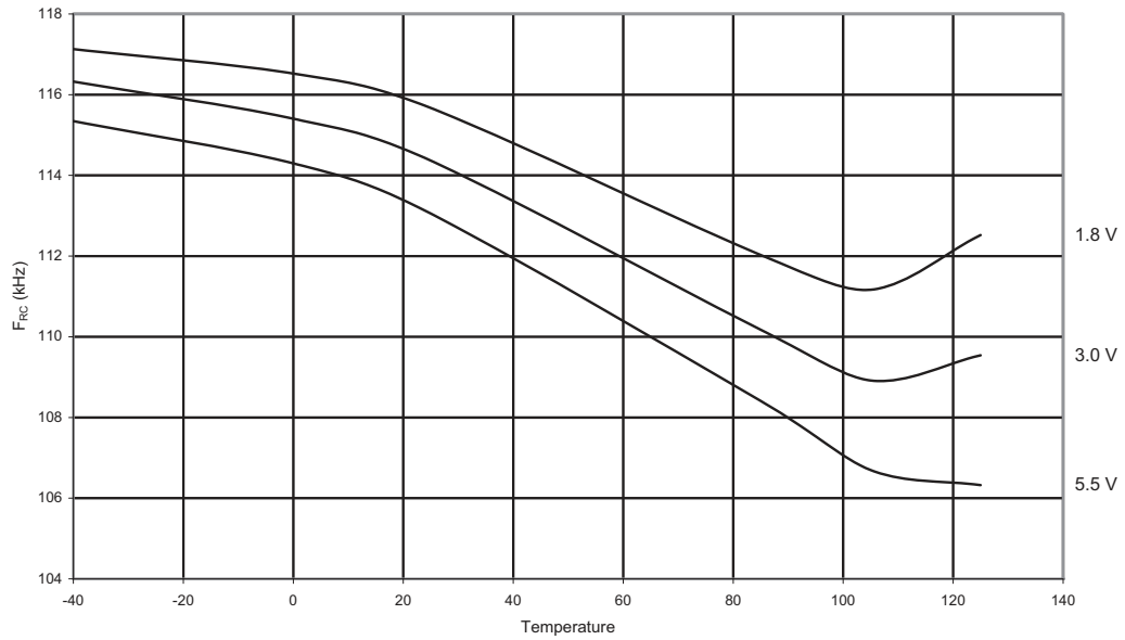
Figure 3-136. Calibrated 8 MHz RC Oscillator Frequency vs. V CC
