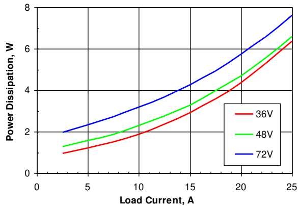
Figure 4. Power dissipation vs. load current and input voltage for SSQE48T25015 converter mounted vertically with air flowing from pin 1 to pin 3 at a rate of 300 LFM (1.5 m/s) and Ta = 25 °C.
