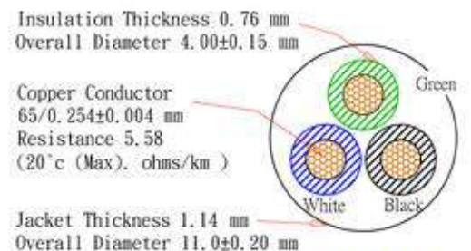
線材截面圖 (Wire Cross-Section)
